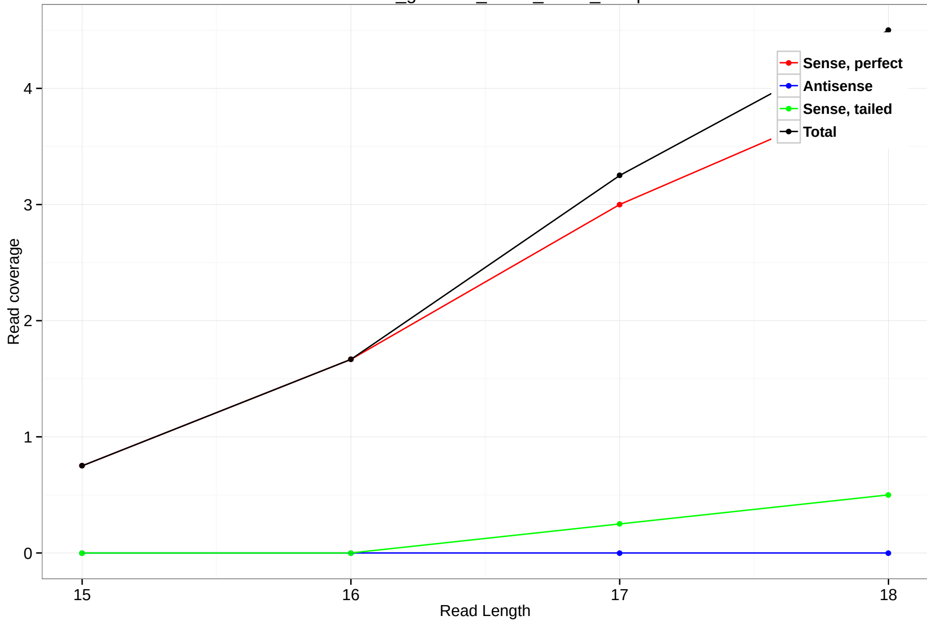
rheMac3_genscan_chr13_08.46_11.3p
