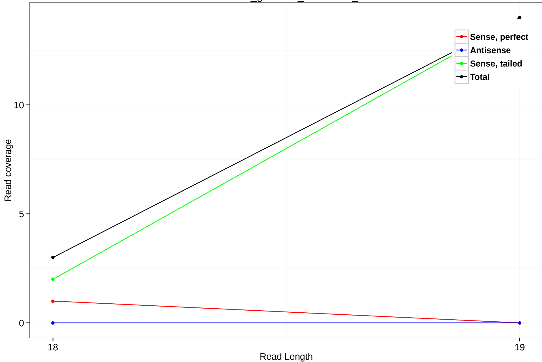
rheMac3_genscan_chr13.010_1
