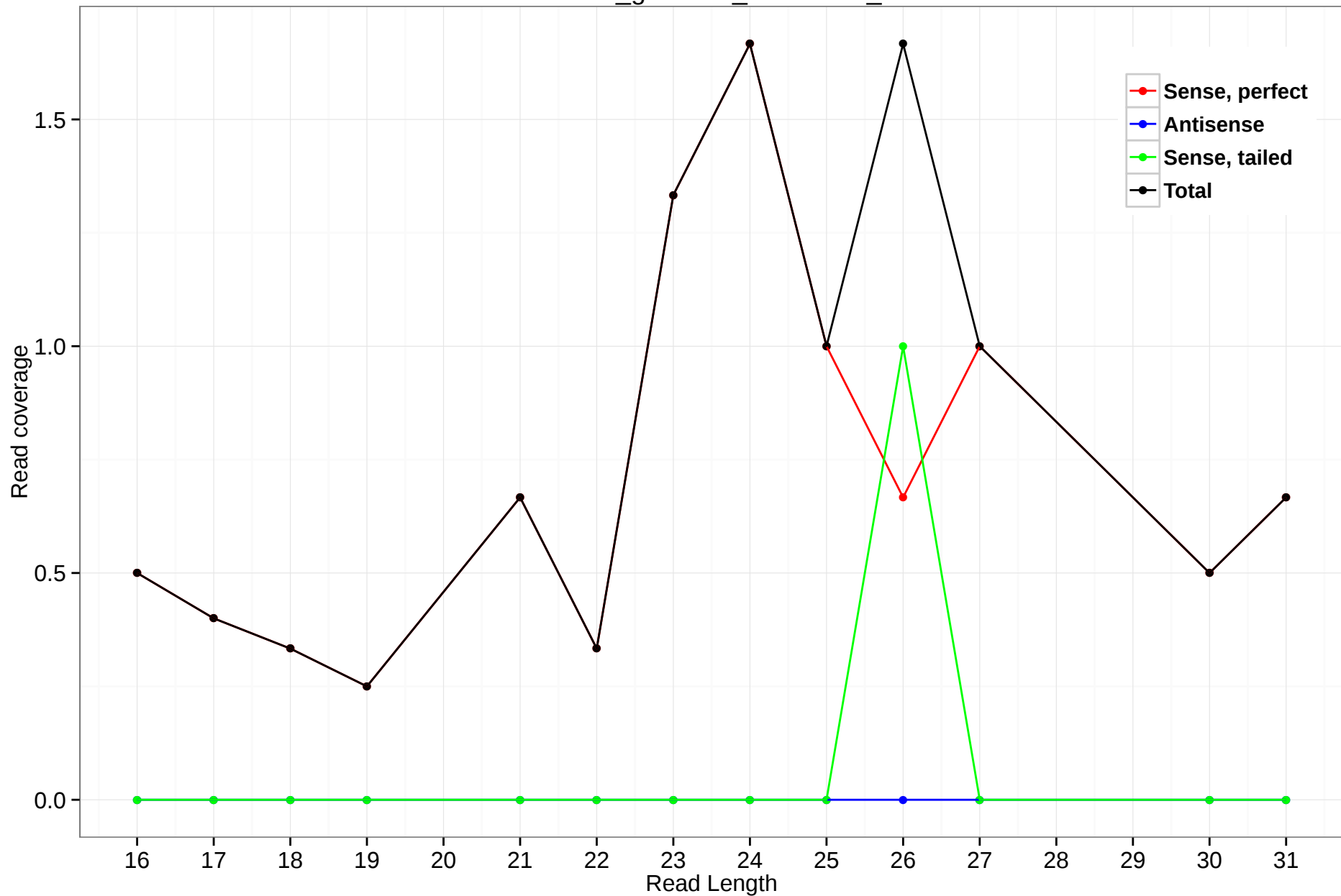
rheMac3_genscan_chr12.870_32
