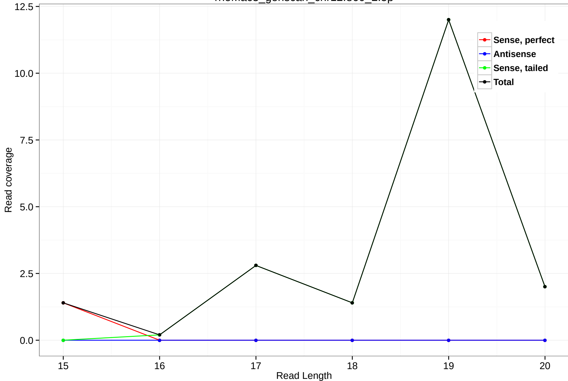
rheMac3_genscan_chr12.860_2.5p
