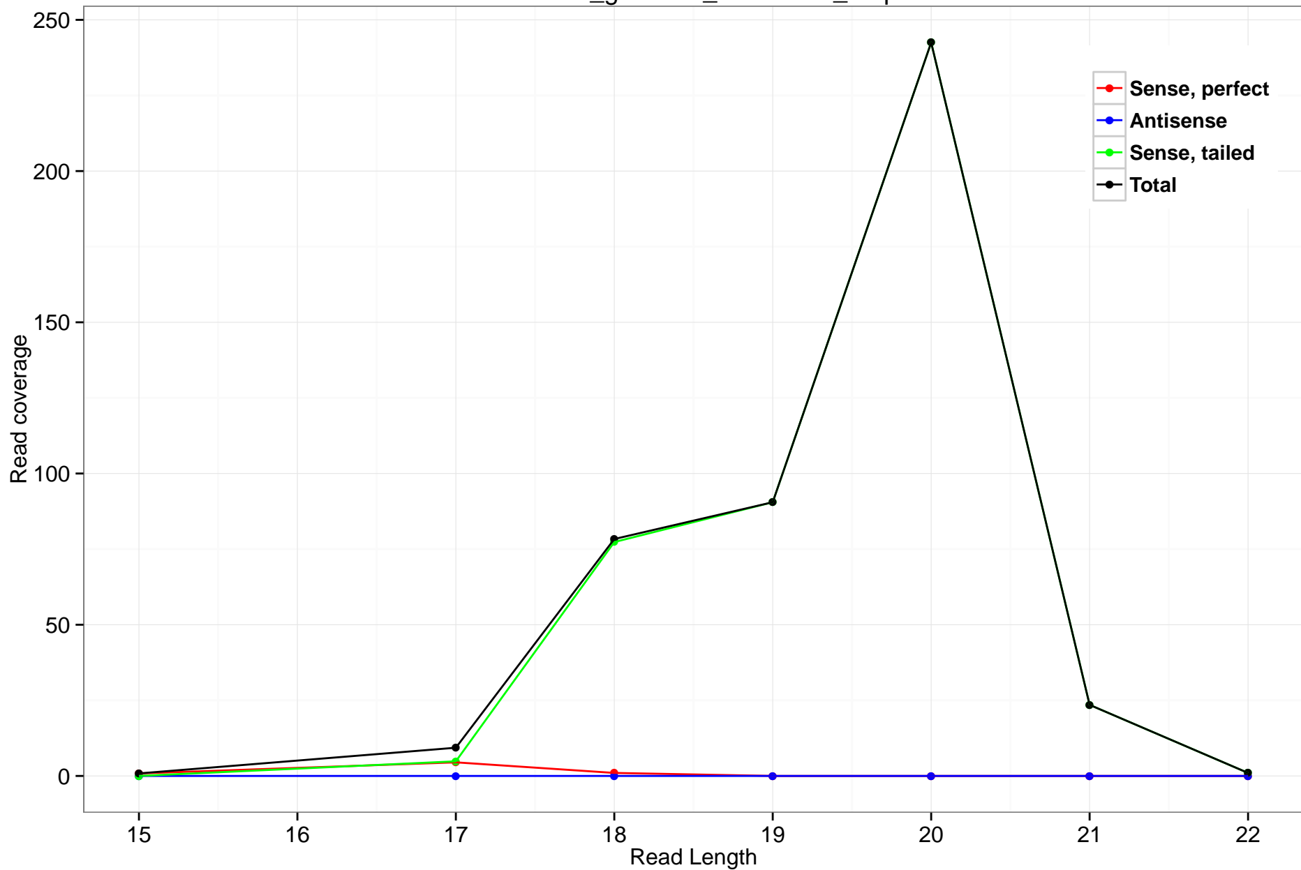
rheMac3_genscan_chr12.858_5.5p
