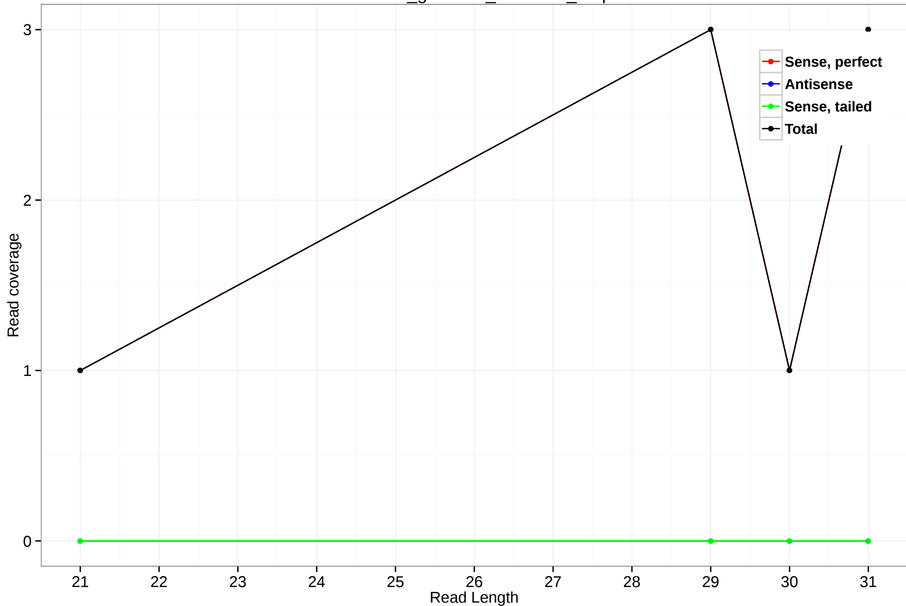
rheMac3_genscan_chr12.81_3.5p
