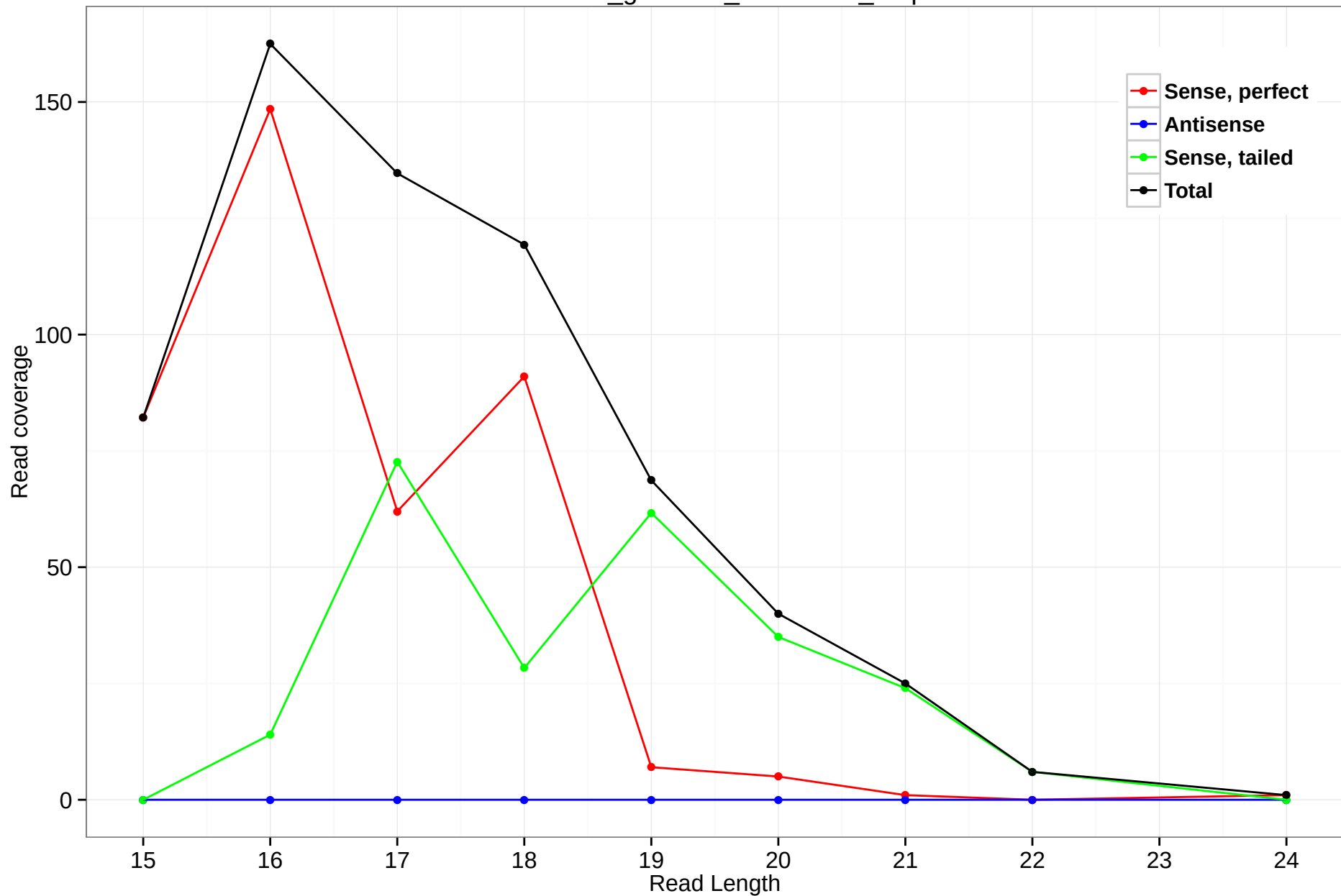
rheMac3_genscan_chr12.743_4.3p
