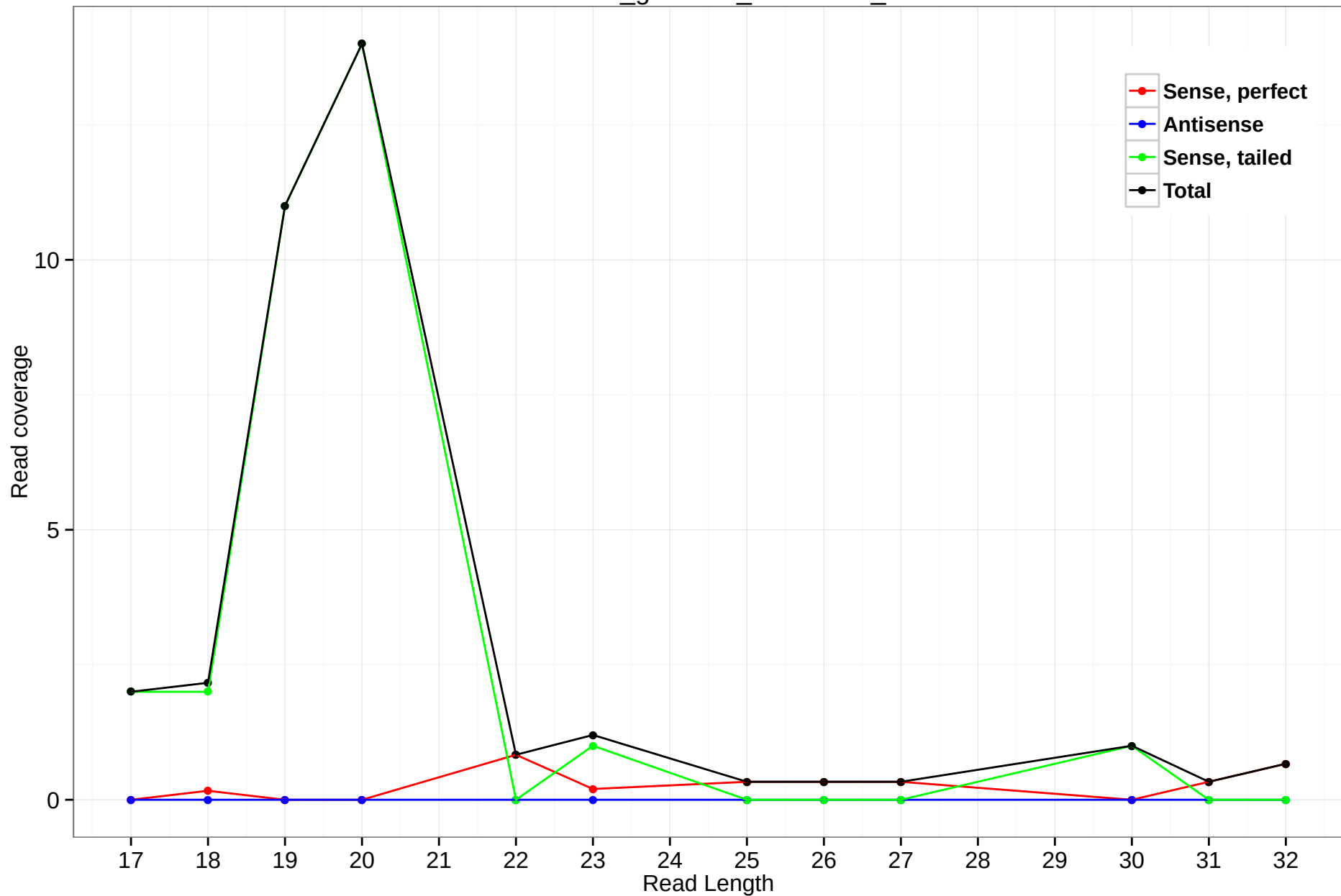
rheMac3_genscan_chr12.678_5
