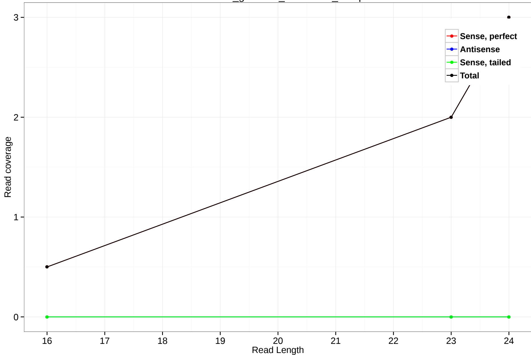
rheMac3_genscan_chr12.552_12.3p
