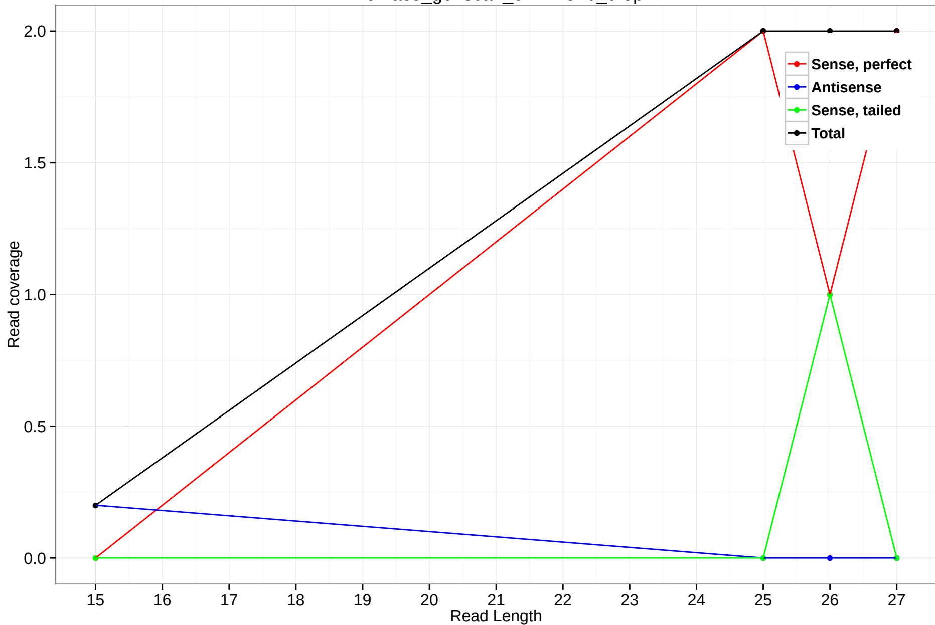
rheMac3_genscan_chr12.510_9.3p
