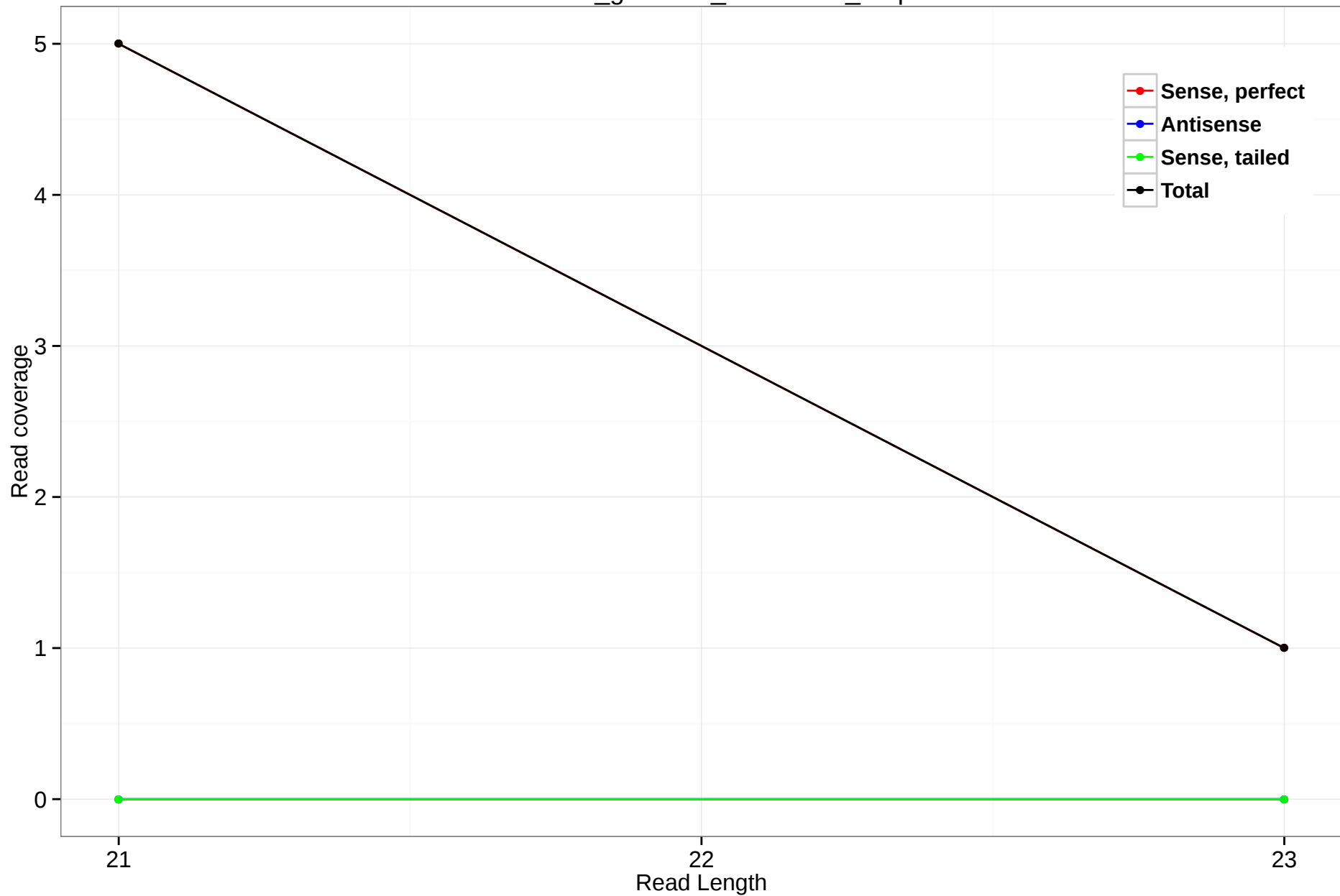
rheMac3_genscan_chr12.510_1.5p
