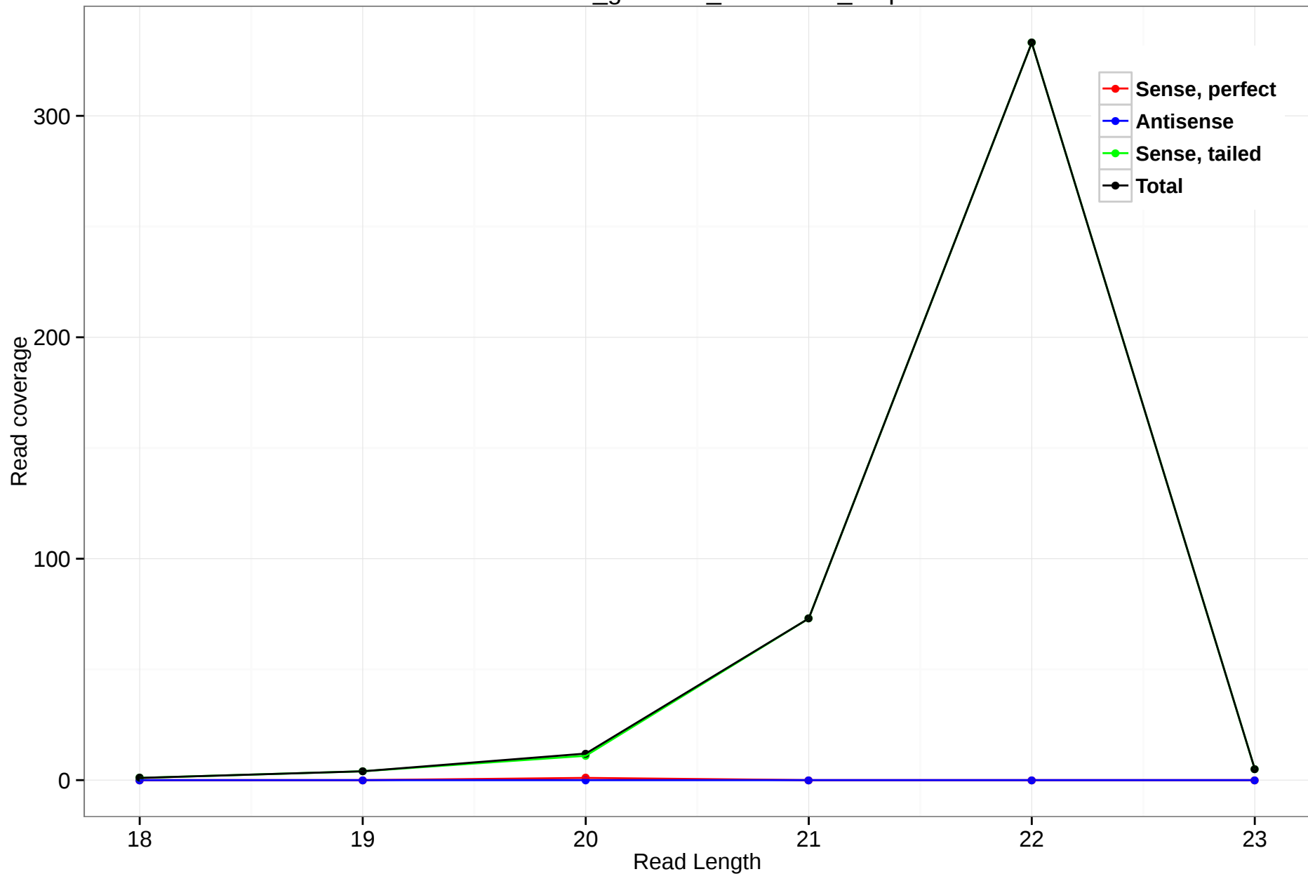
rheMac3_genscan_chr12.506_5.5p
