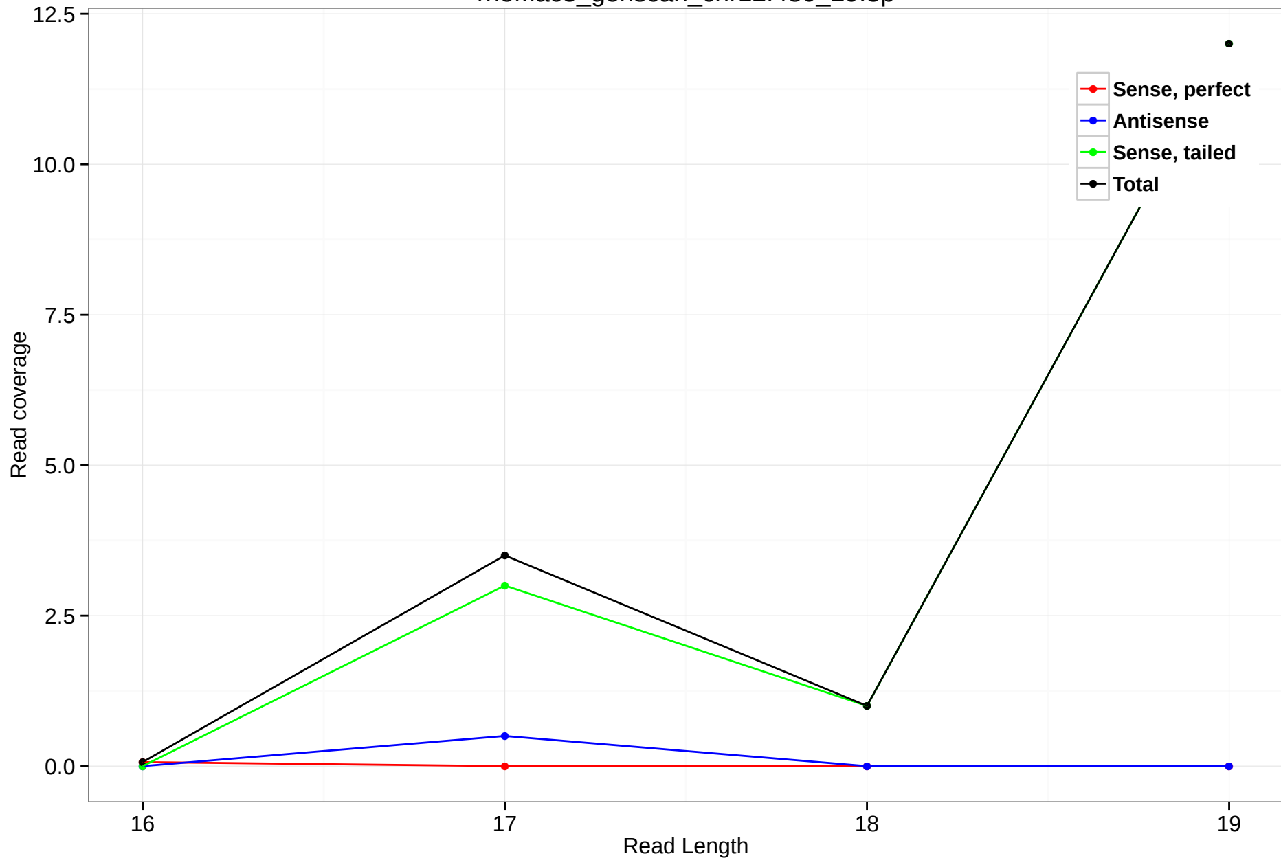
rheMac3_genscan_chr12.480_29.3p
