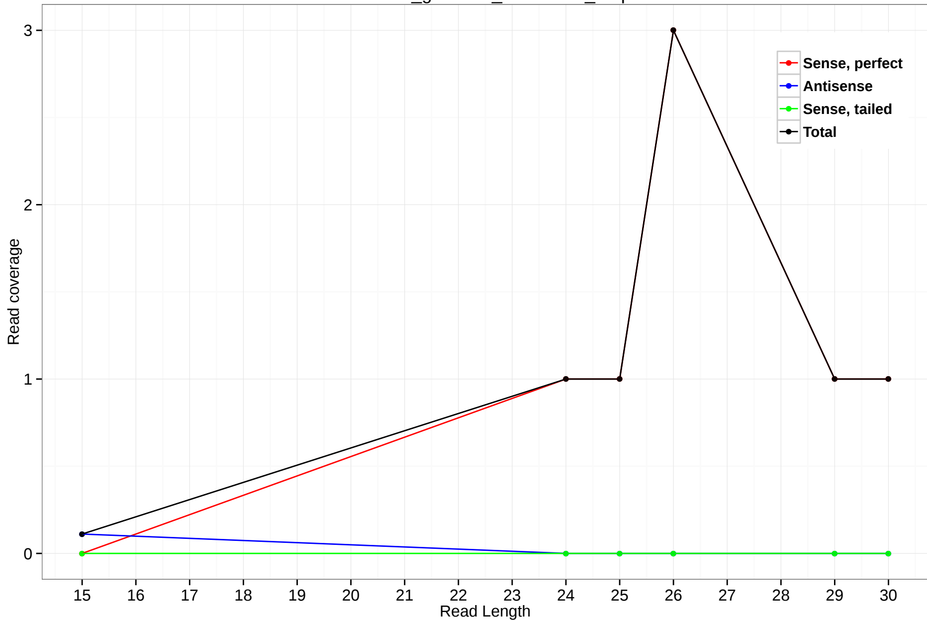
rheMac3_genscan_chr12.411_0.3p
