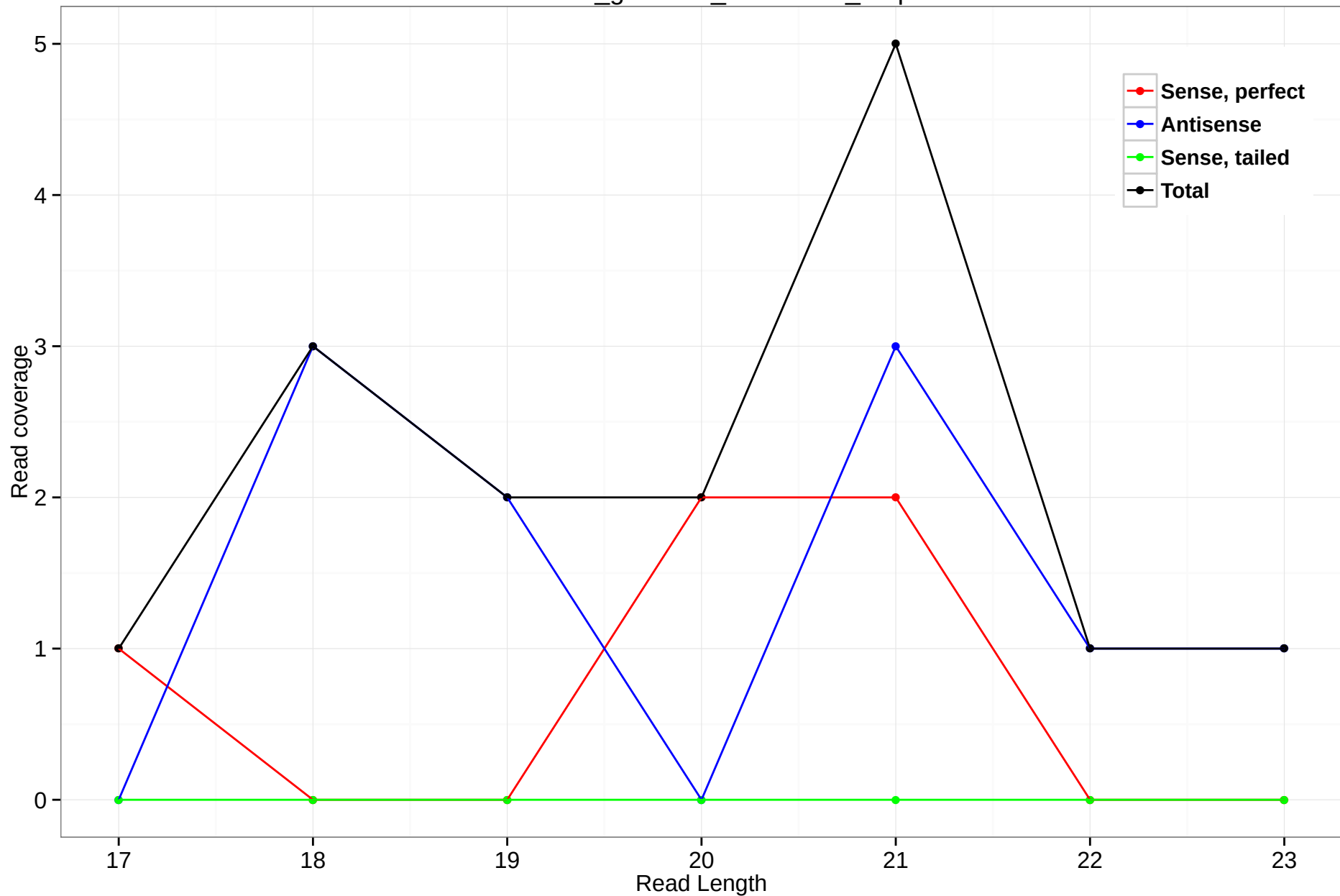
rheMac3_genscan_chr12.399_3.5p
