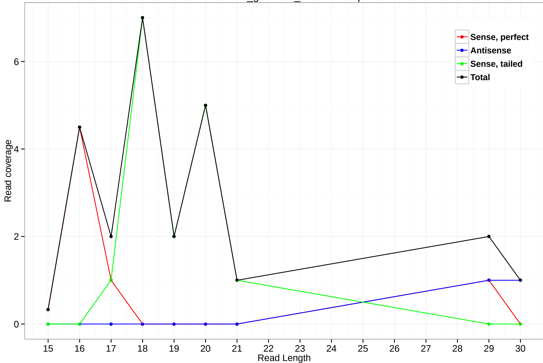
rheMac3_genscan_chr12.391.3p
