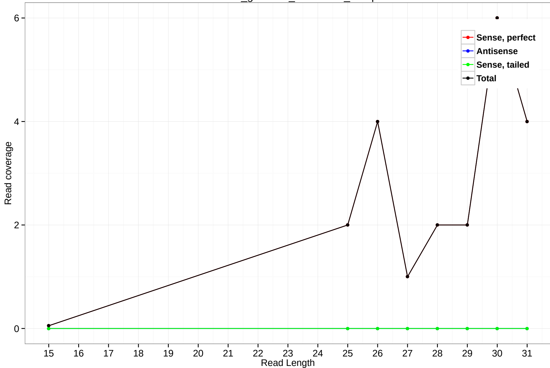
rheMac3_genscan_chr12.338_17.5p
