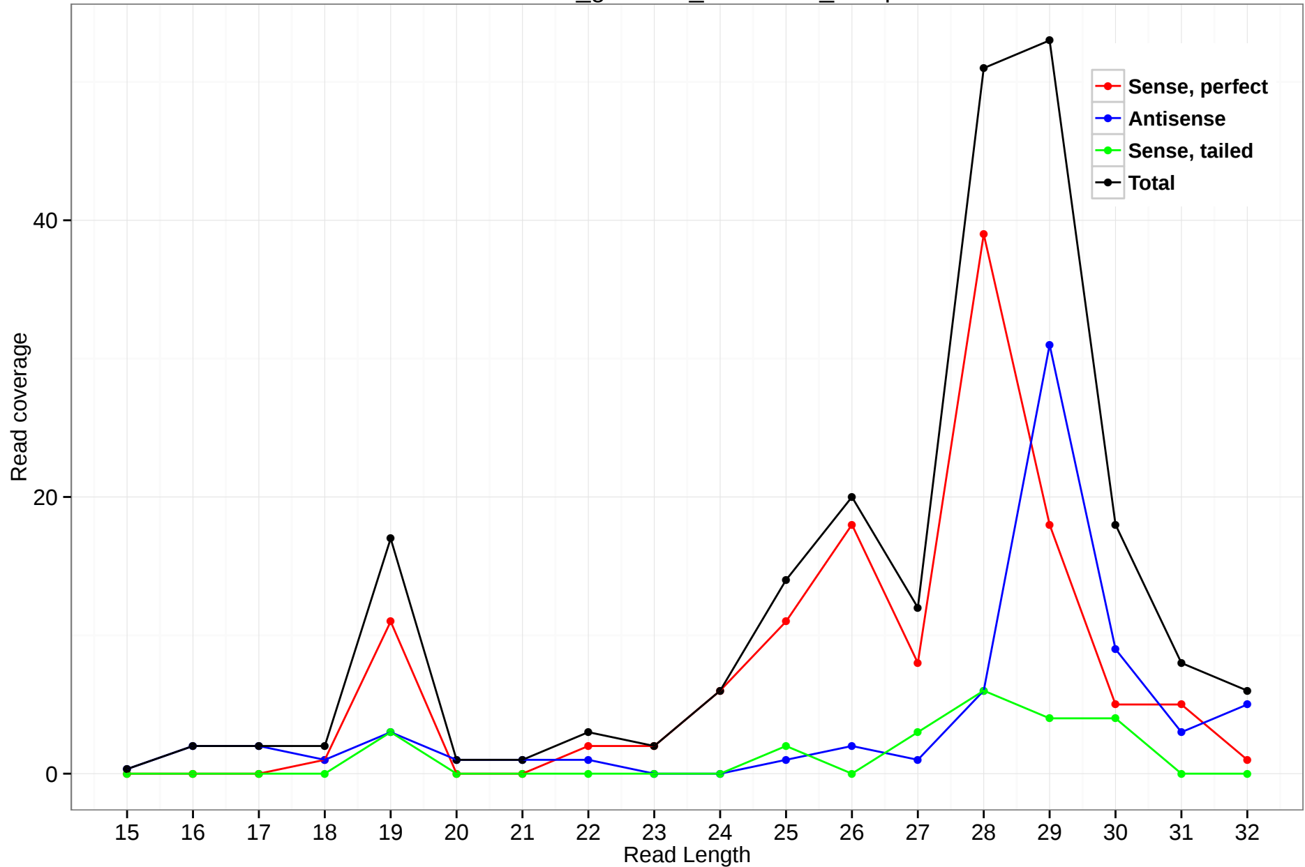
rheMac3_genscan_chr12.338_14.5p
