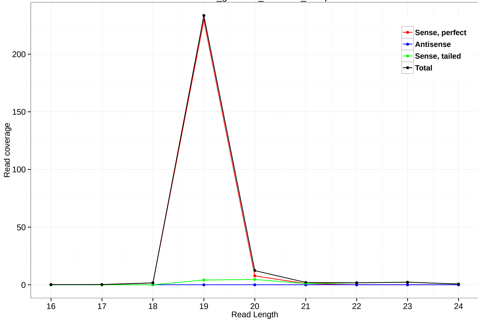
rheMac3_genscan_chr12.28_25.3p
