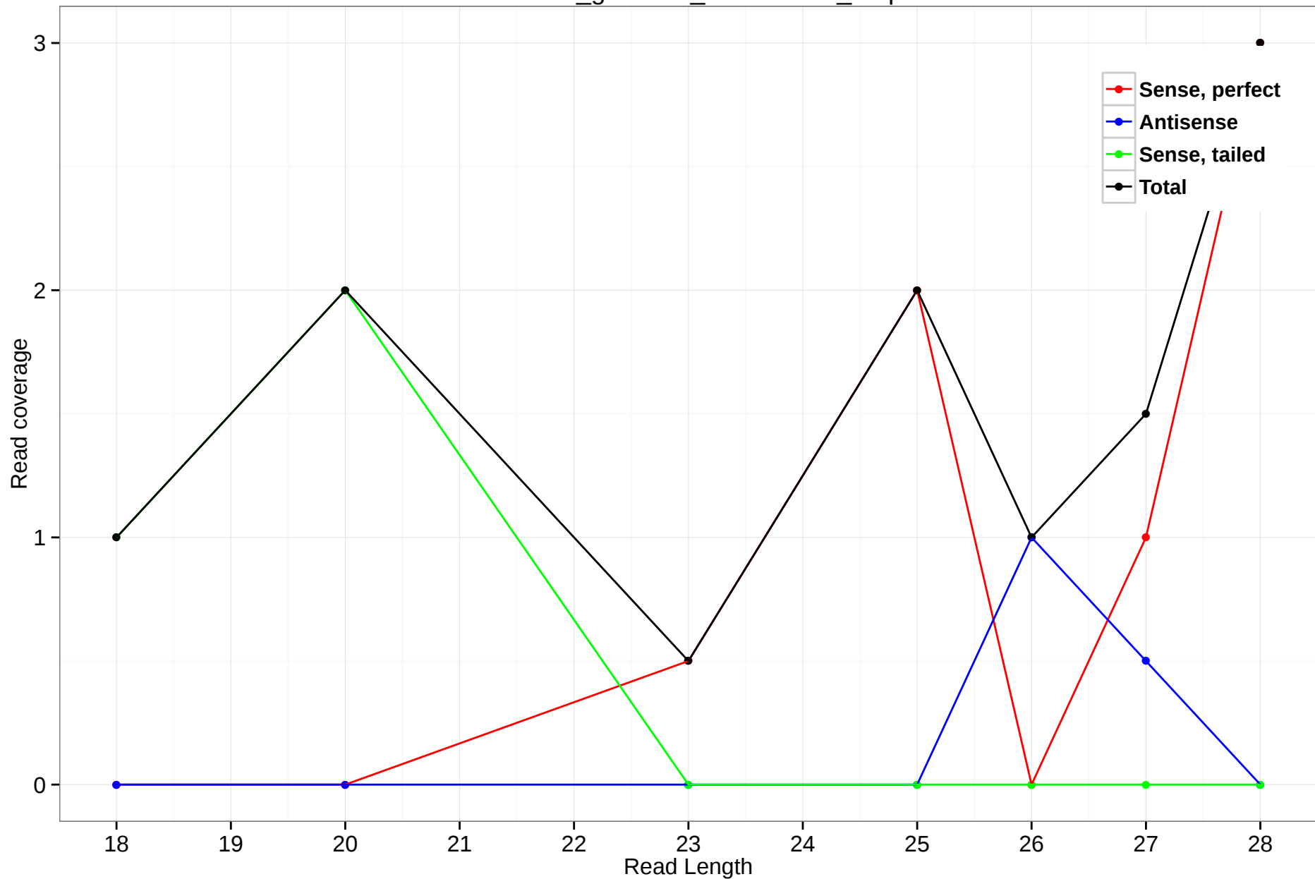
rheMac3_genscan_chr12.1991_0.5p
