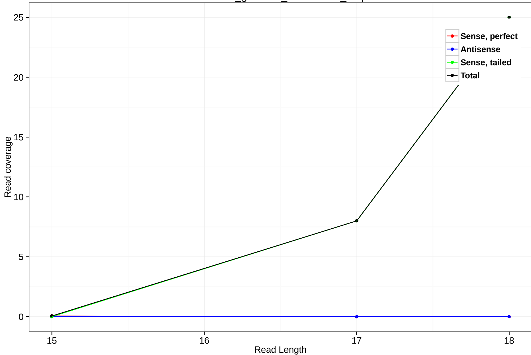
rheMac3_genscan_chr12.1936_9.3p
