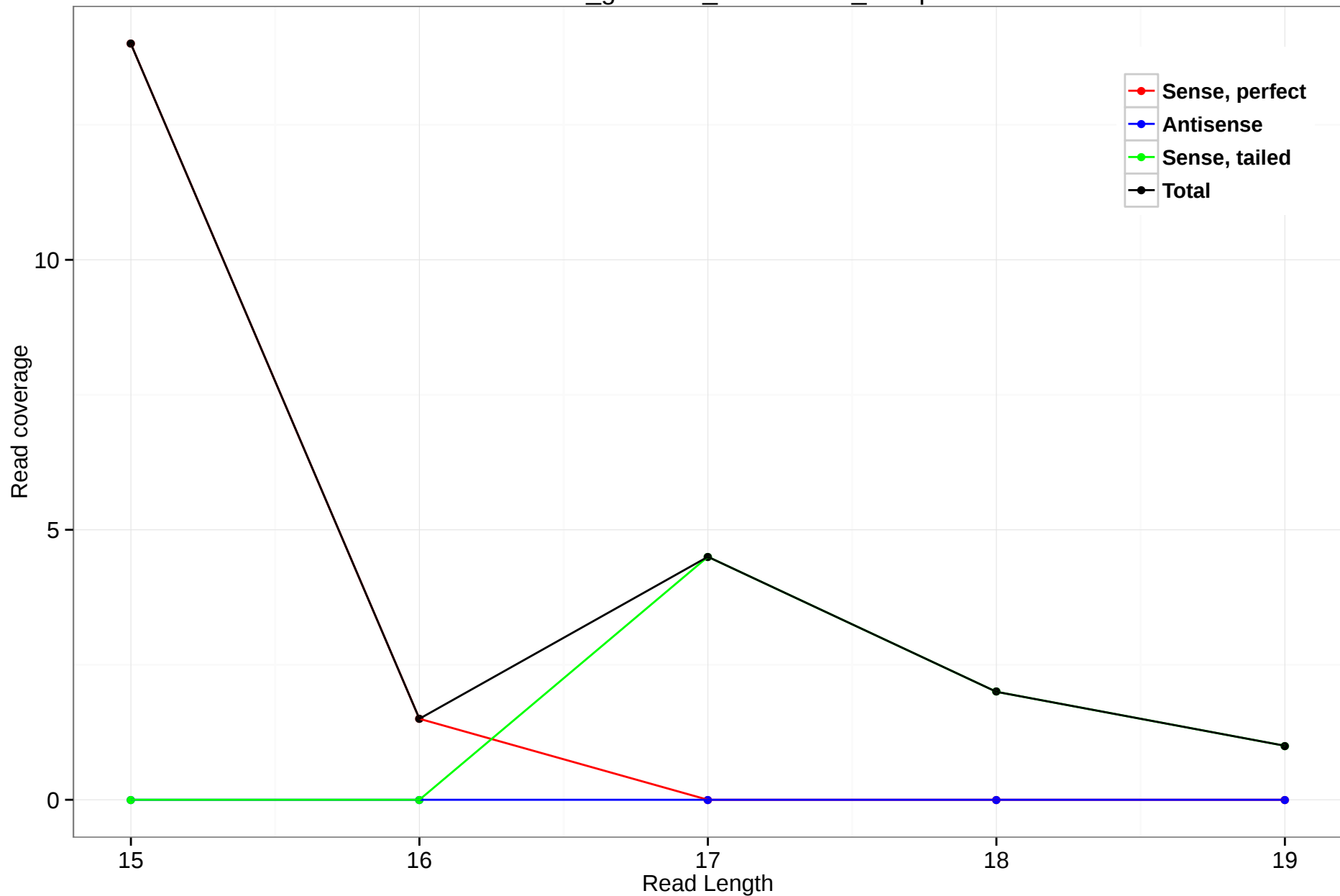
rheMac3_genscan_chr12.1936_48.3p
