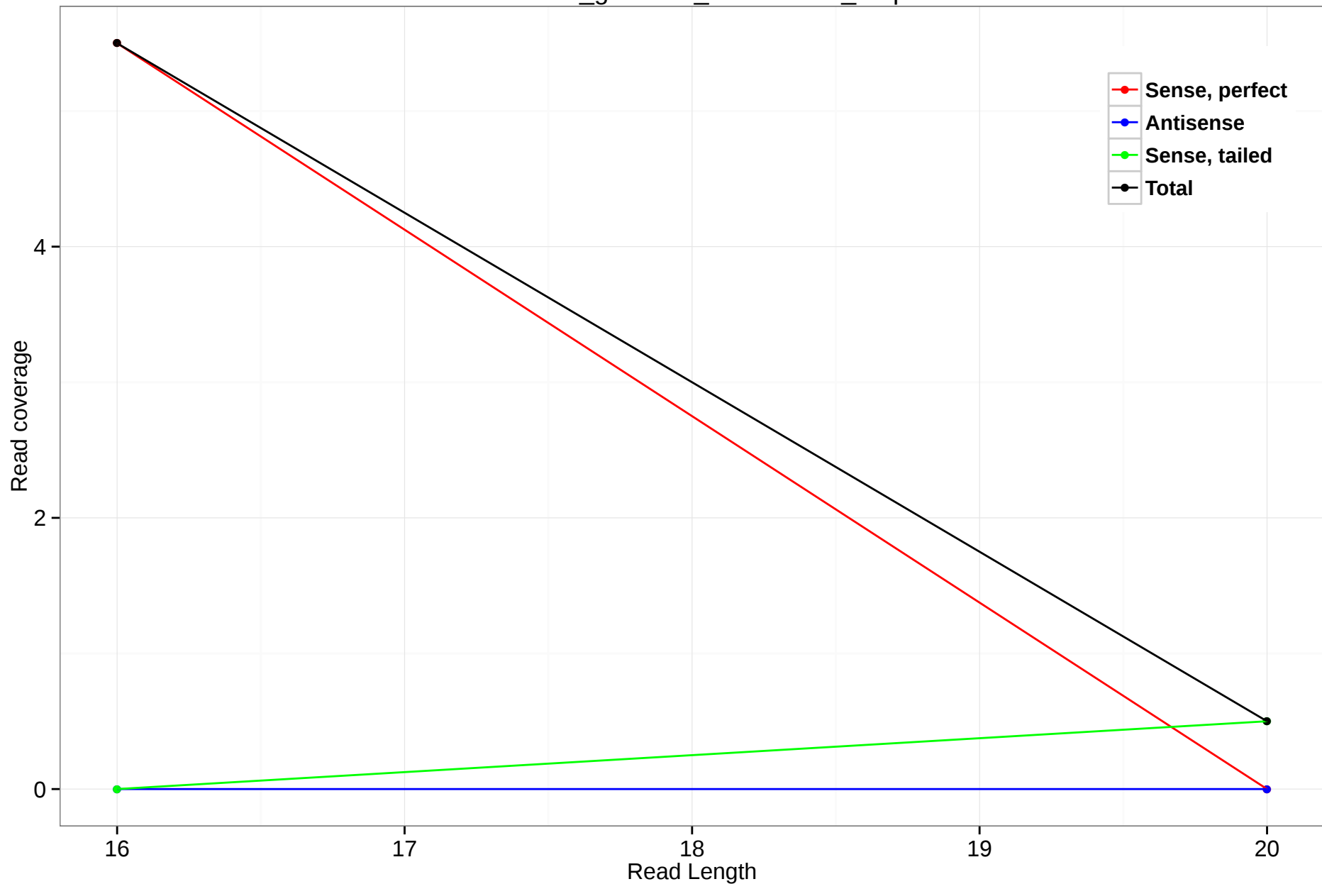
rheMac3_genscan_chr12.1926_0.3p
