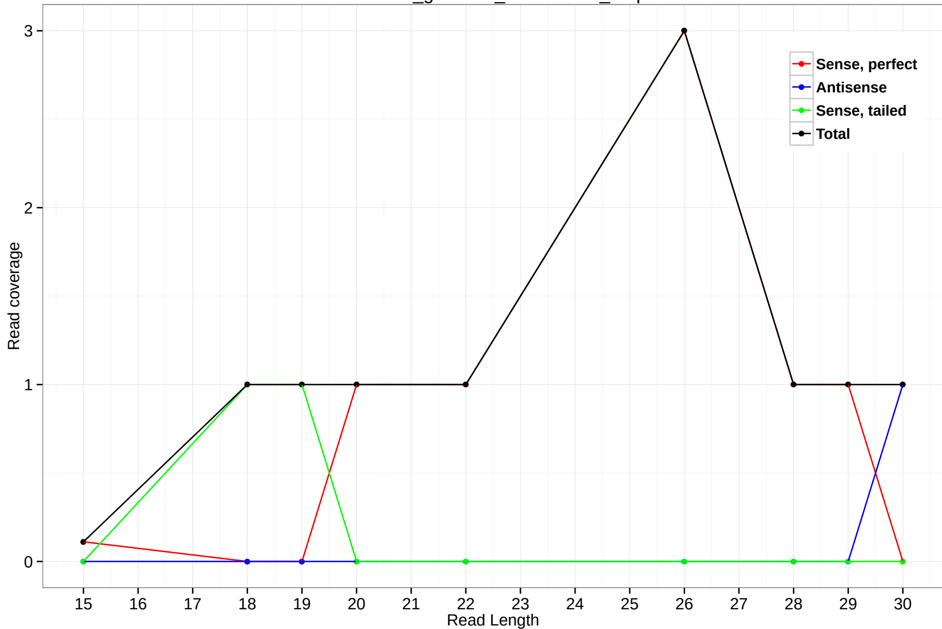
rheMac3_genscan_chr12.1900_2.5p
