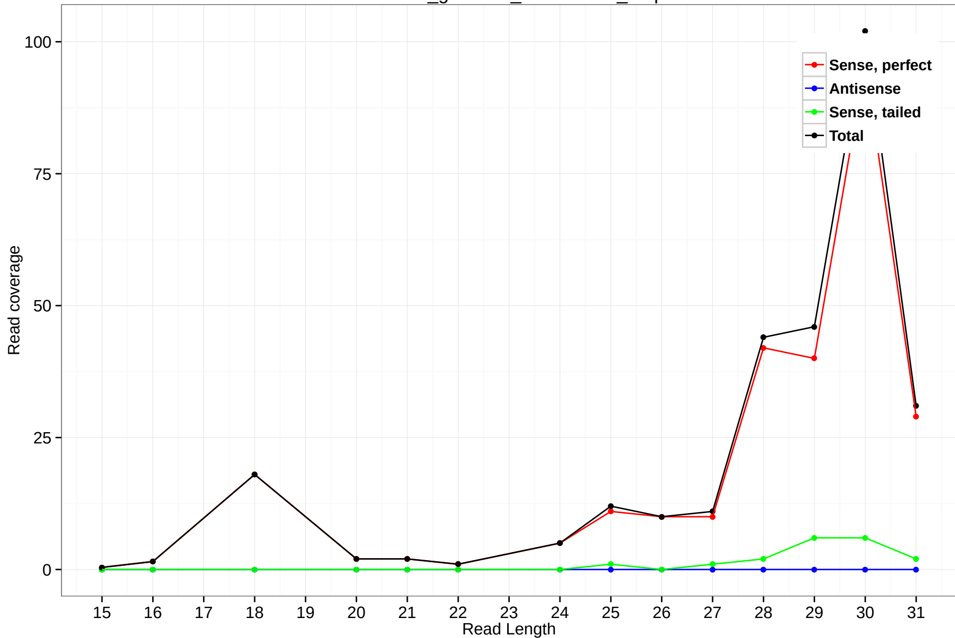
rheMac3_genscan_chr12.1883_5.5p
