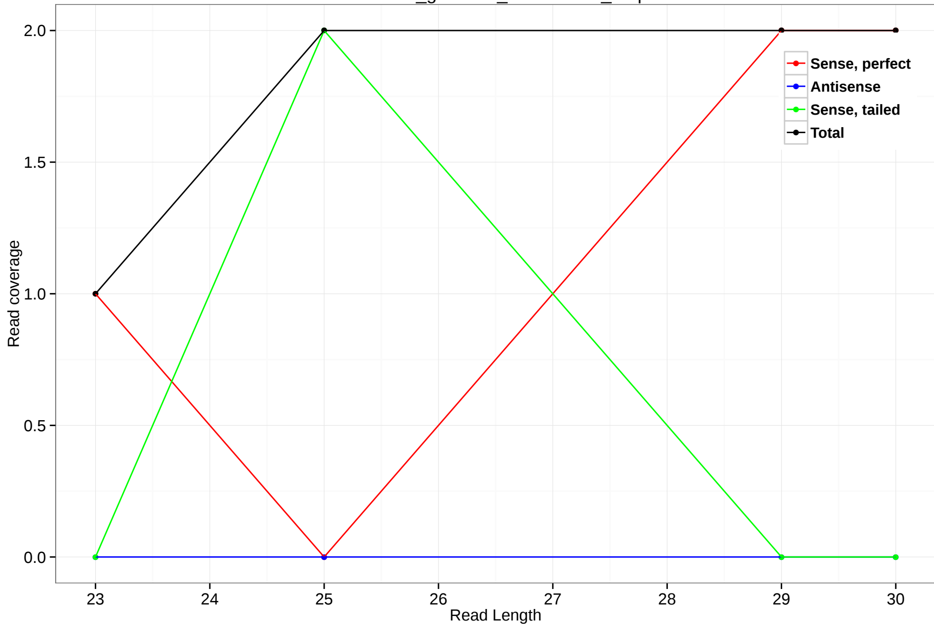
rheMac3_genscan_chr12.1858_0.5p
