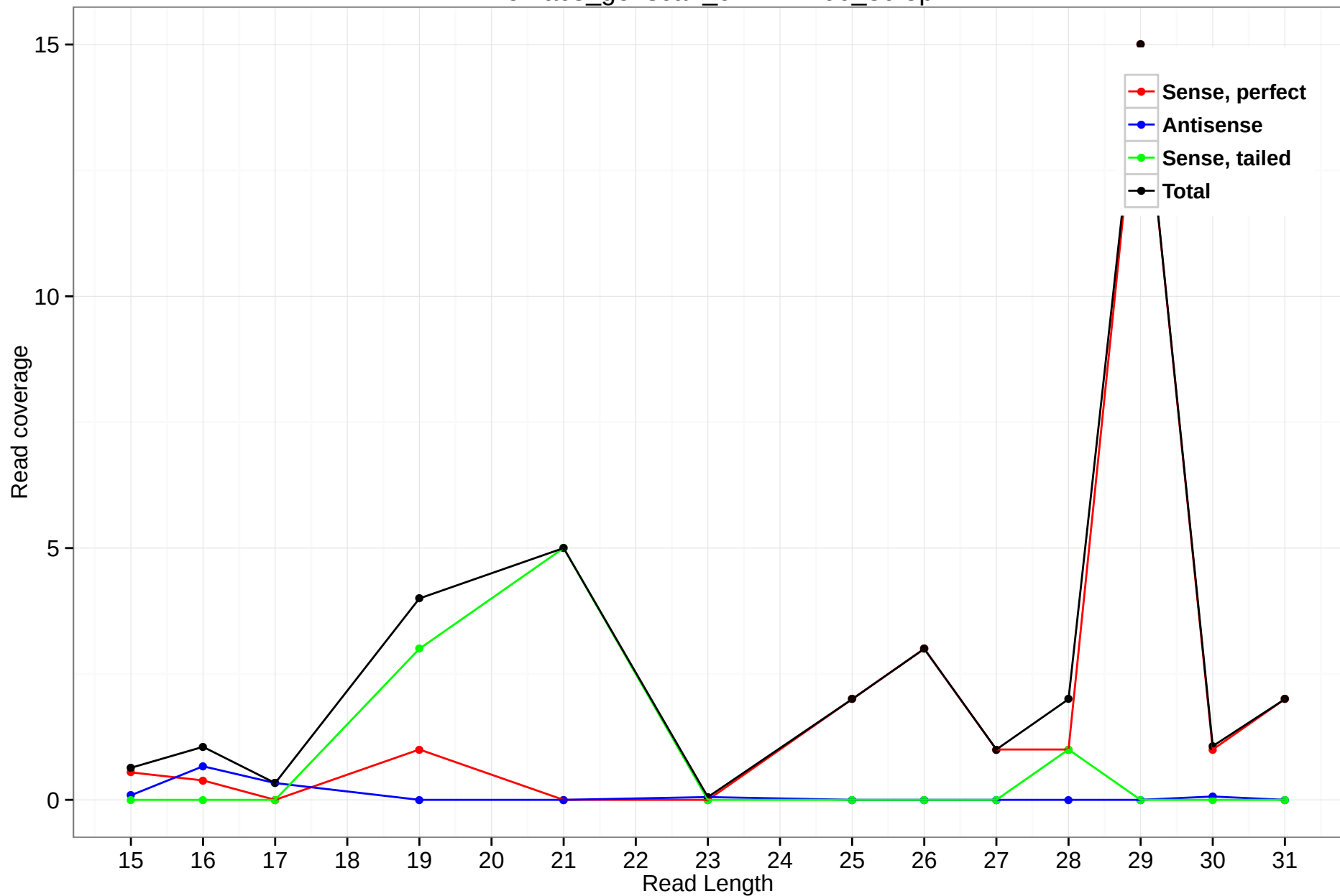
rheMac3_genscan_chr12.1706_30.5p
