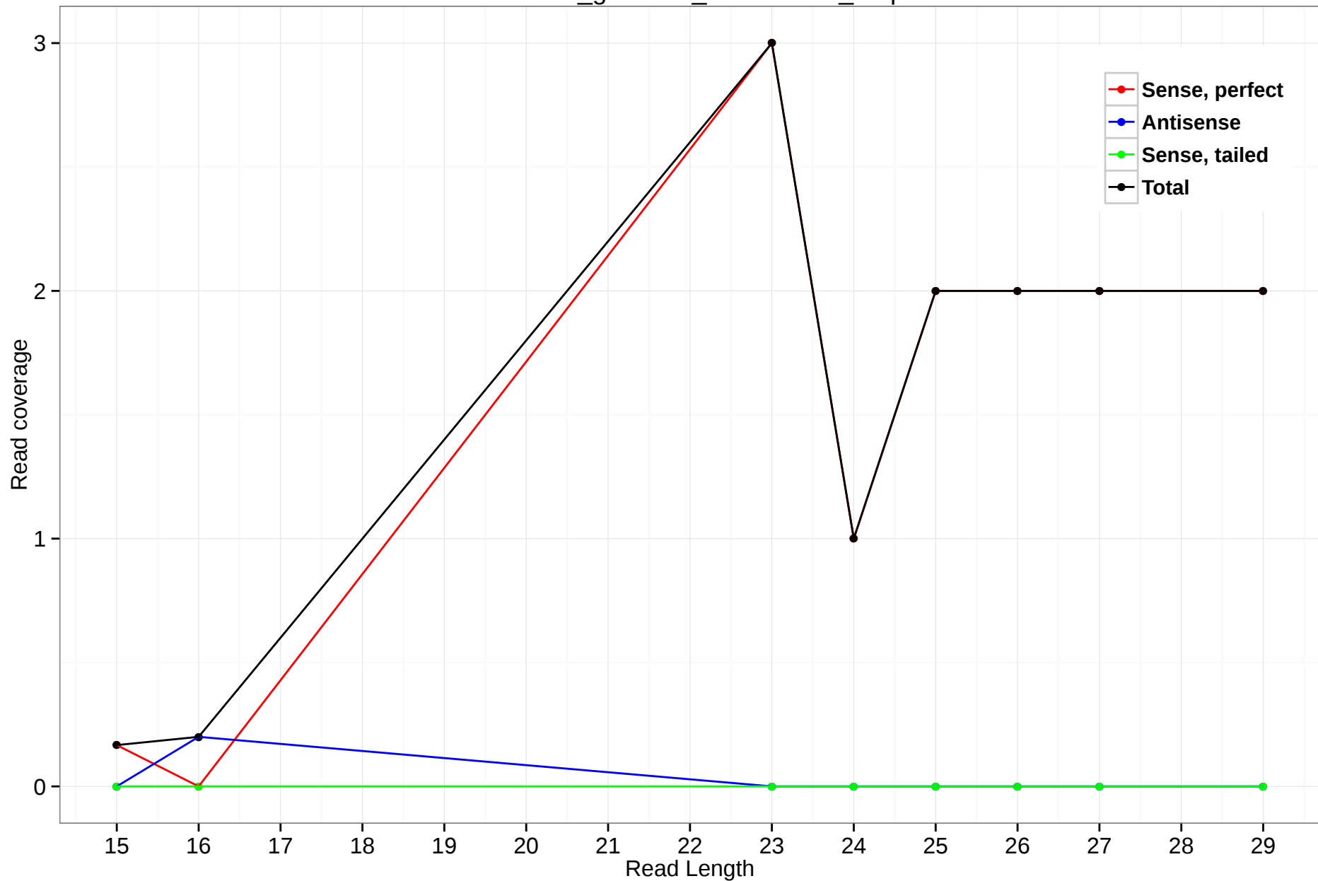
rheMac3_genscan_chr12.1629_6.5p
