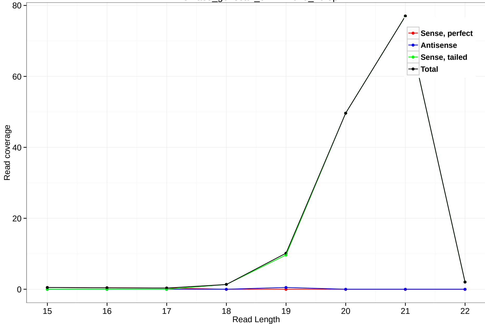
rheMac3_genscan_chr12.1629_20.3p
