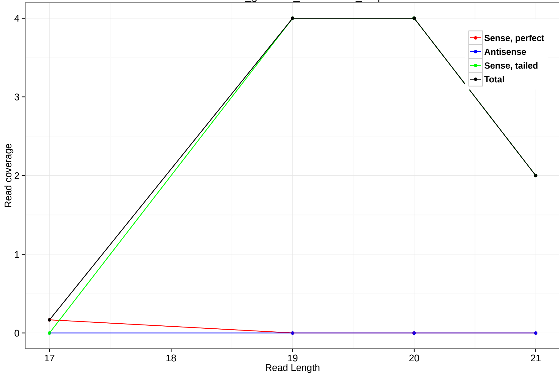
rheMac3_genscan_chr12.1572_6.5p
