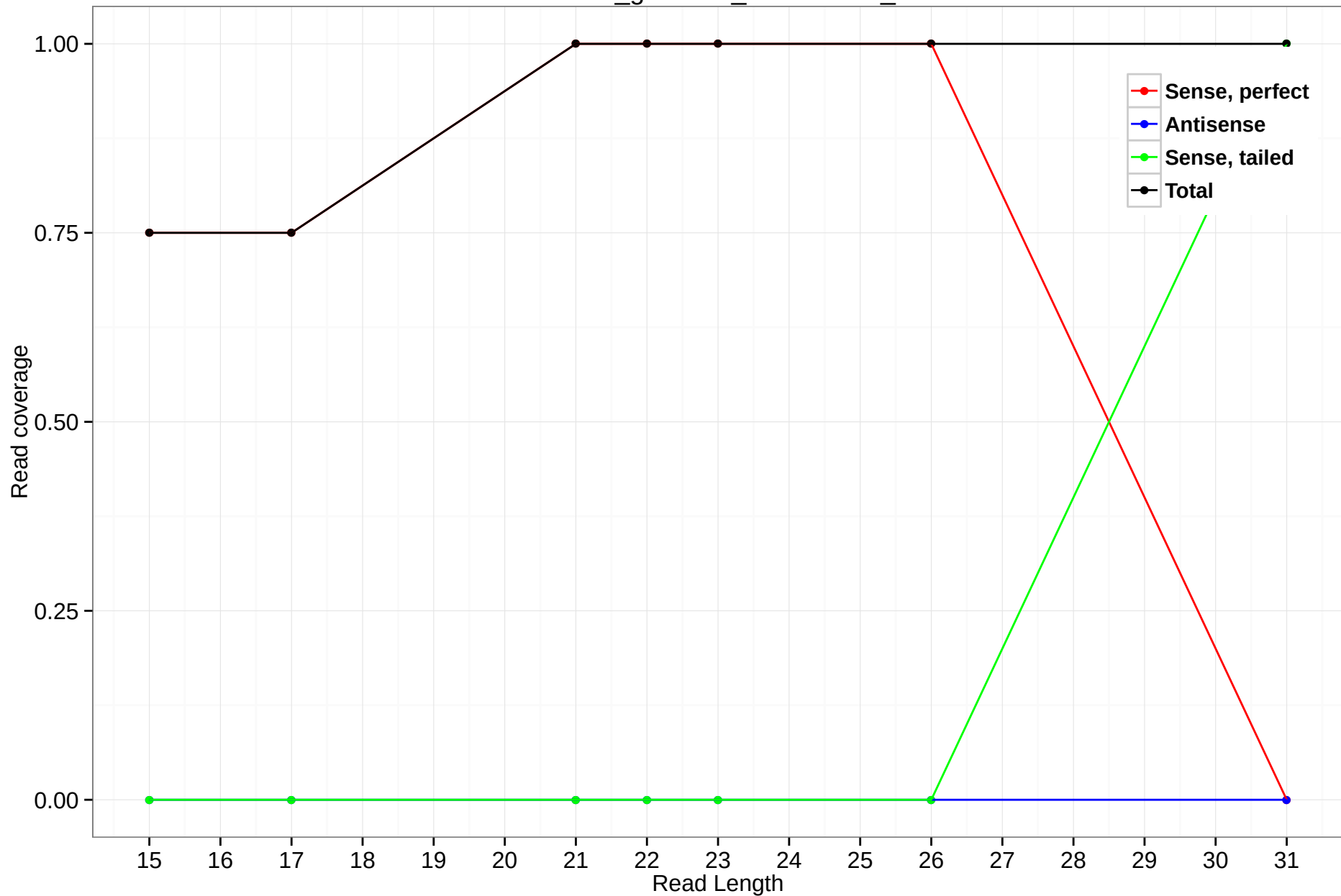
rheMac3_genscan_chr12.1377_32
