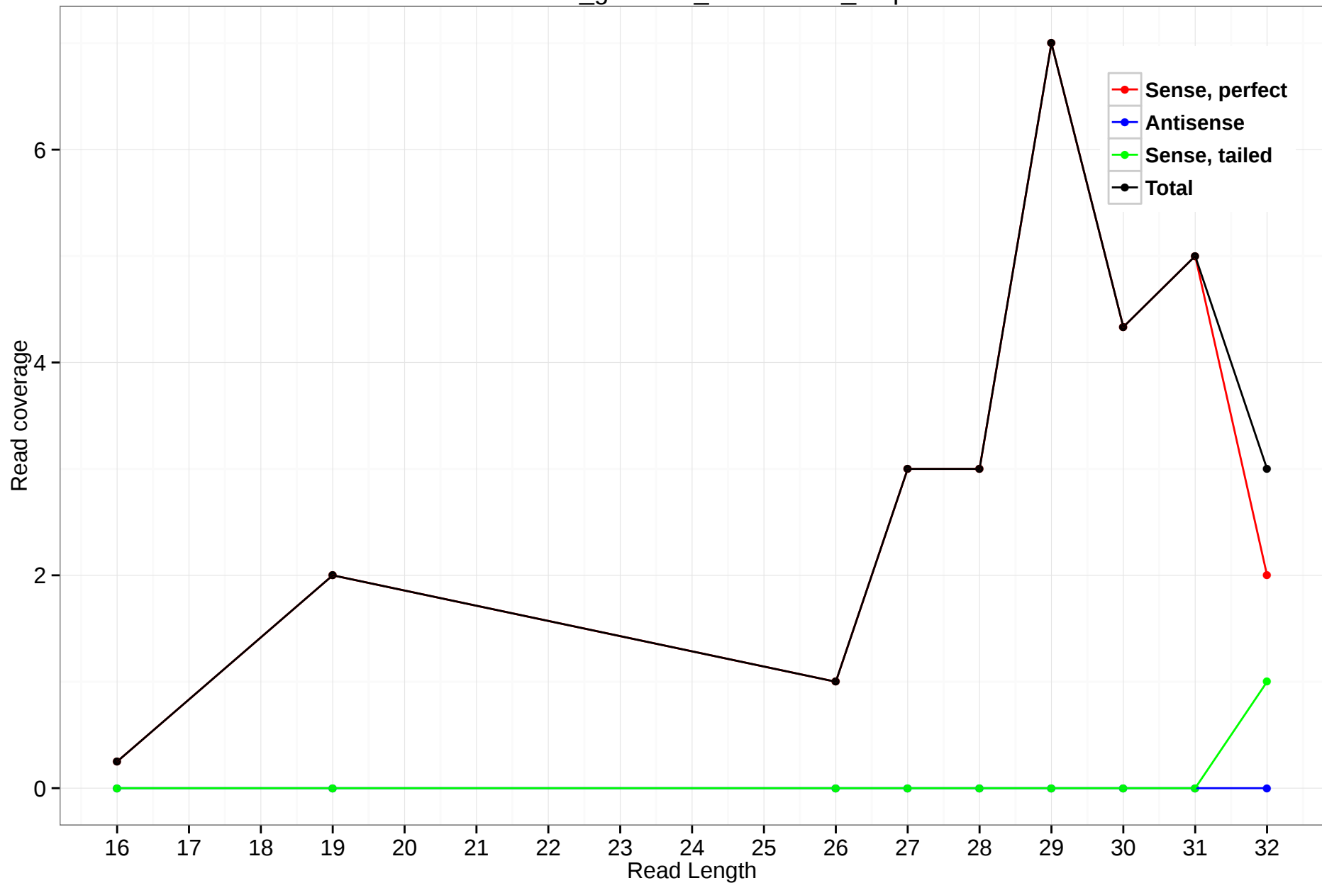
rheMac3_genscan_chr12.1355_7.5p
