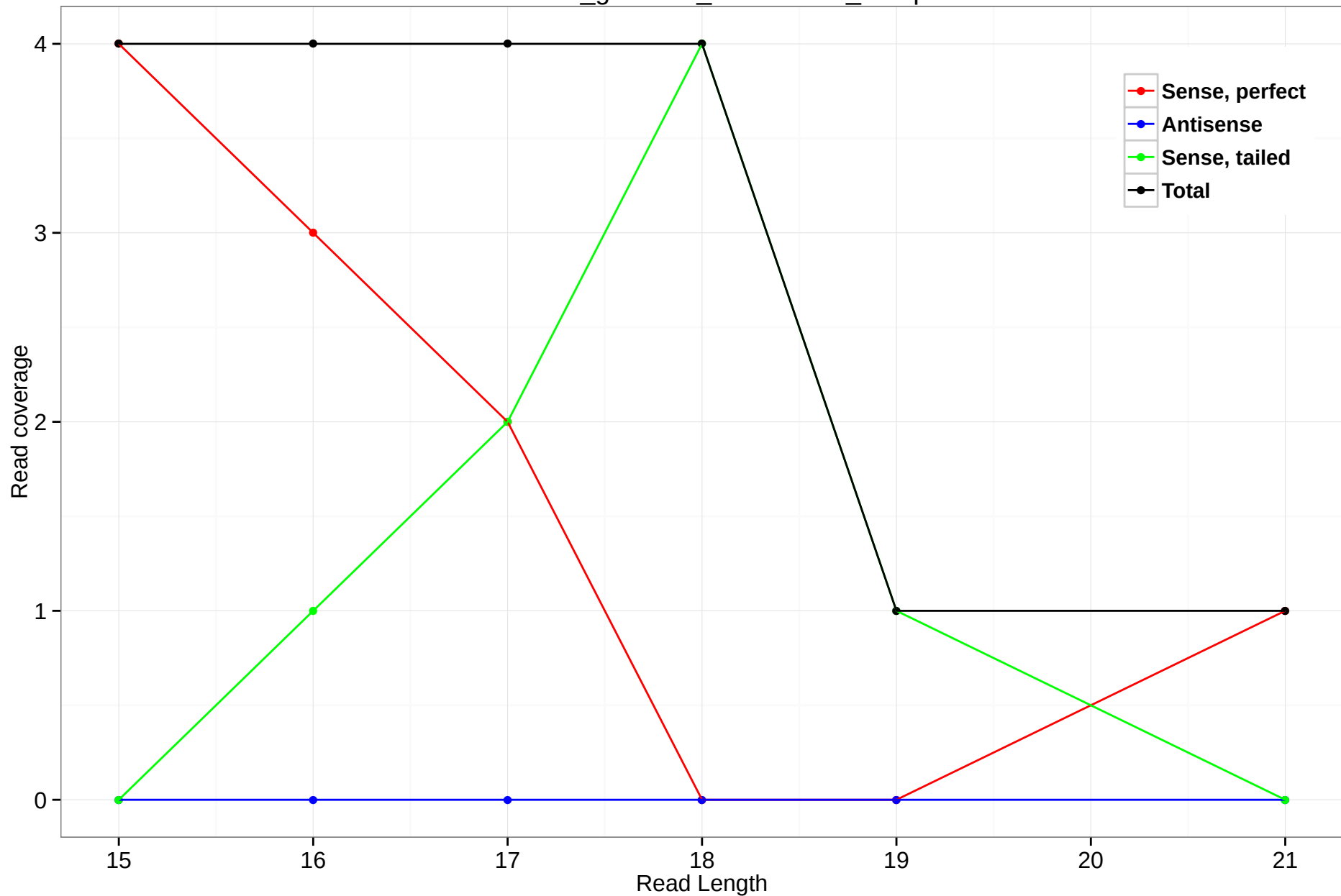
rheMac3_genscan_chr12.1352_28.5p
