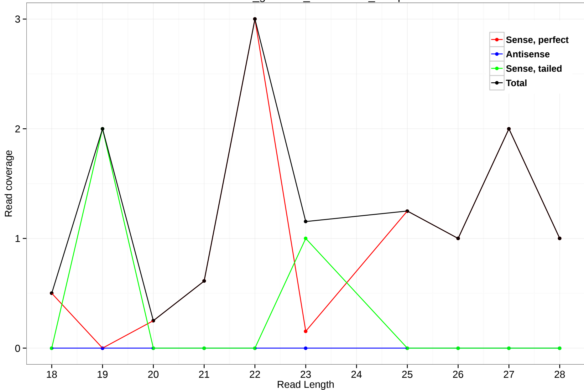
rheMac3_genscan_chr12.1204_12.5p
