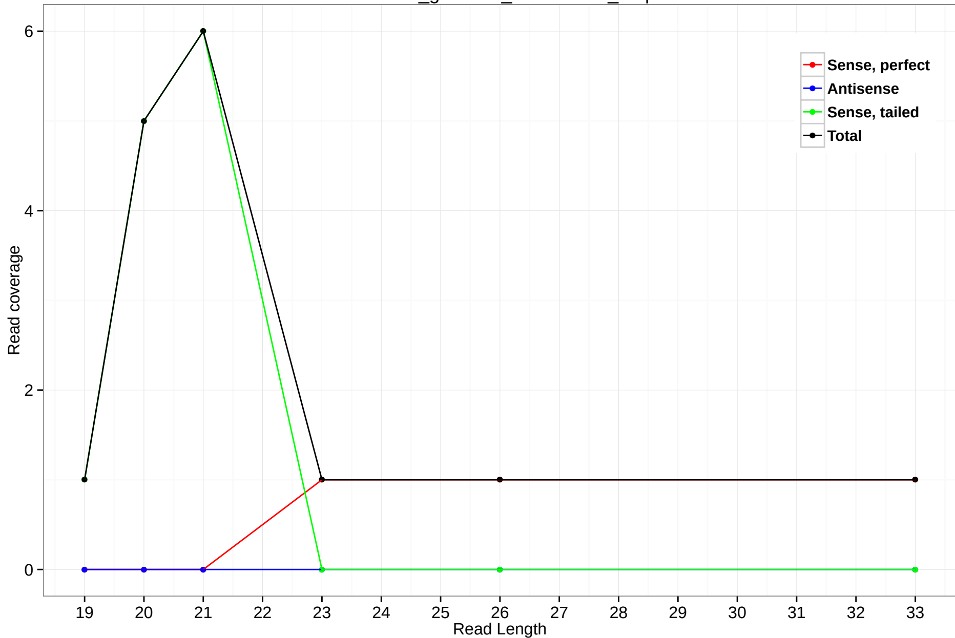
rheMac3_genscan_chr12.1172_1.3p
