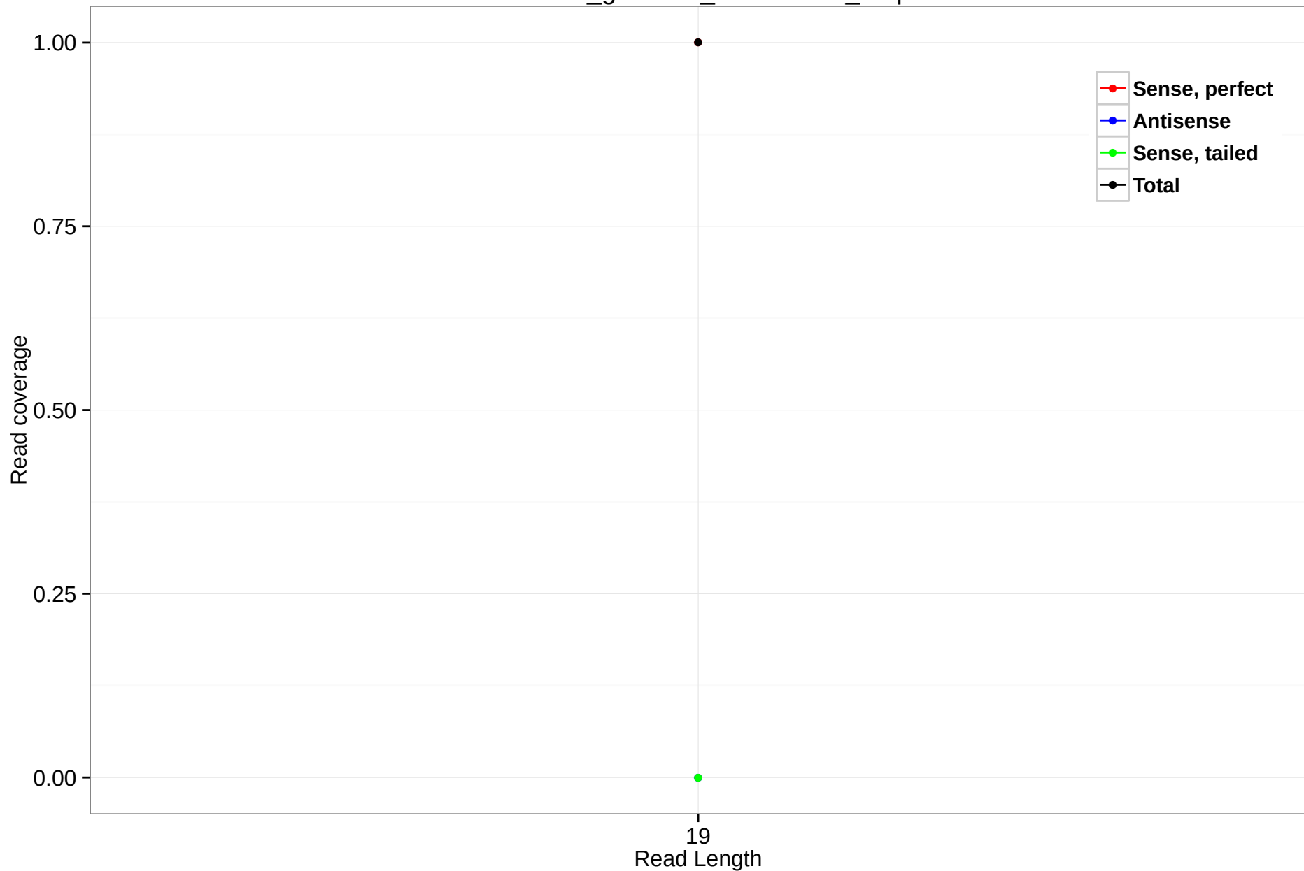
rheMac3_genscan_chr12.1137_6.5p
