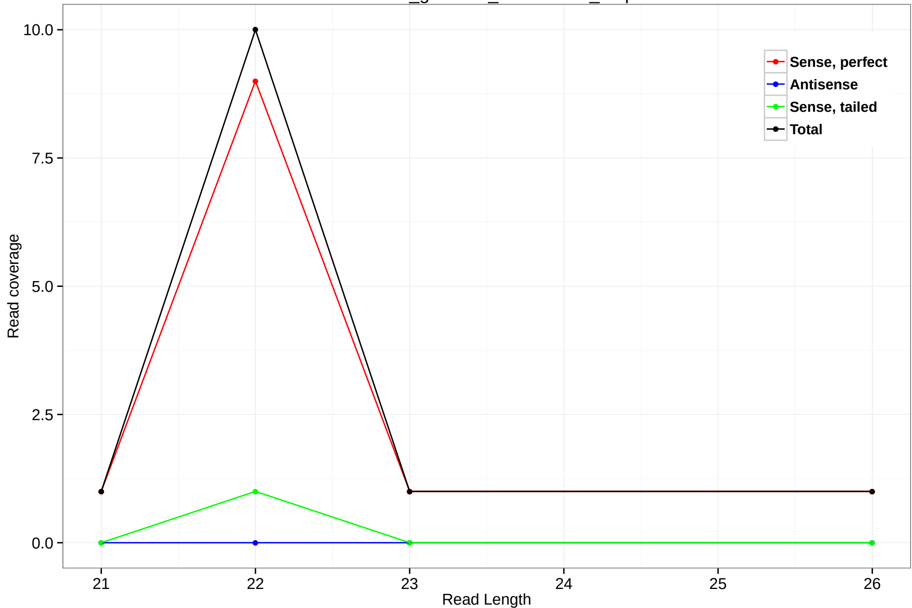
rheMac3_genscan_chr12.1029_0.5p
