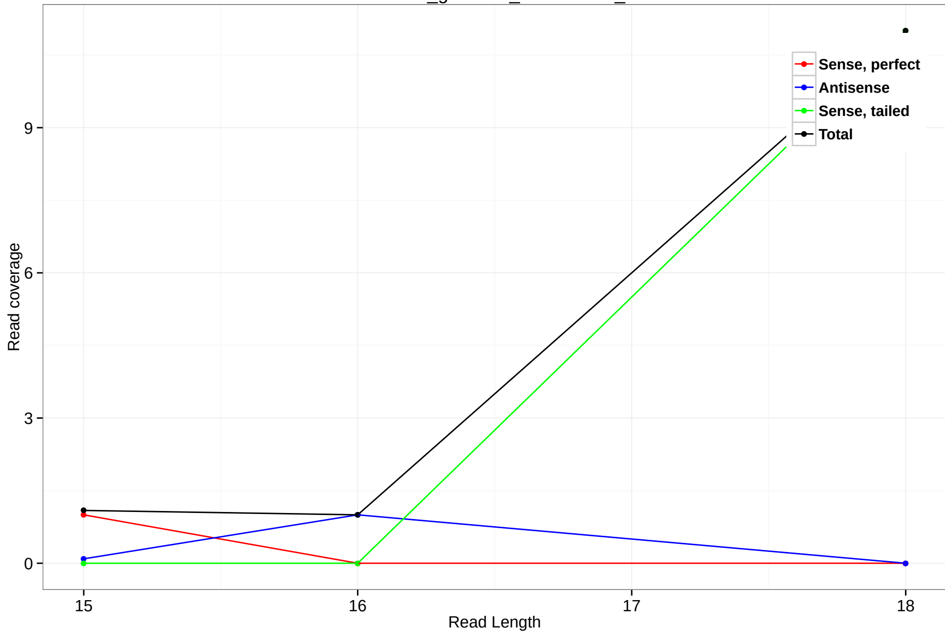
rheMac3_genscan_chr12.1027_1
