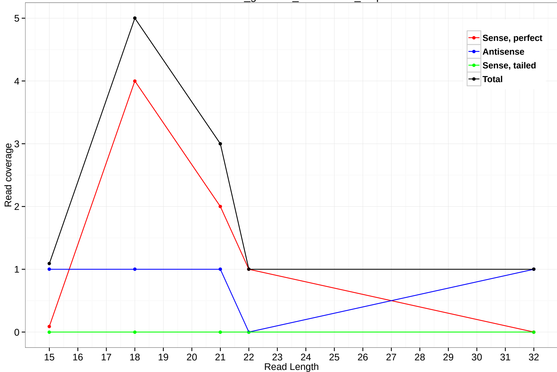
rheMac3_genscan_chr12.1019_1.5p
