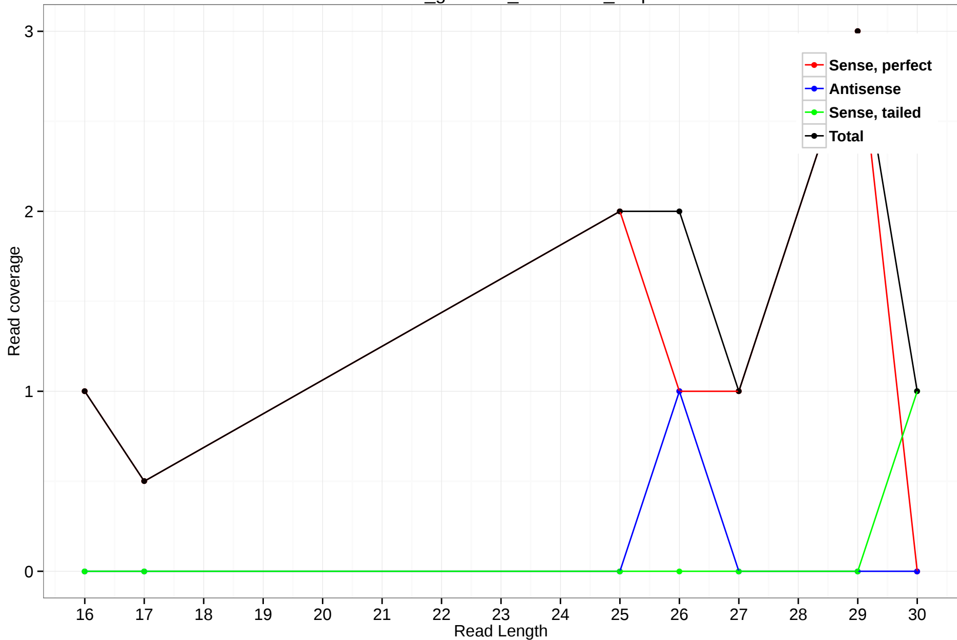
rheMac3_genscan_chr11.989_3.3p
