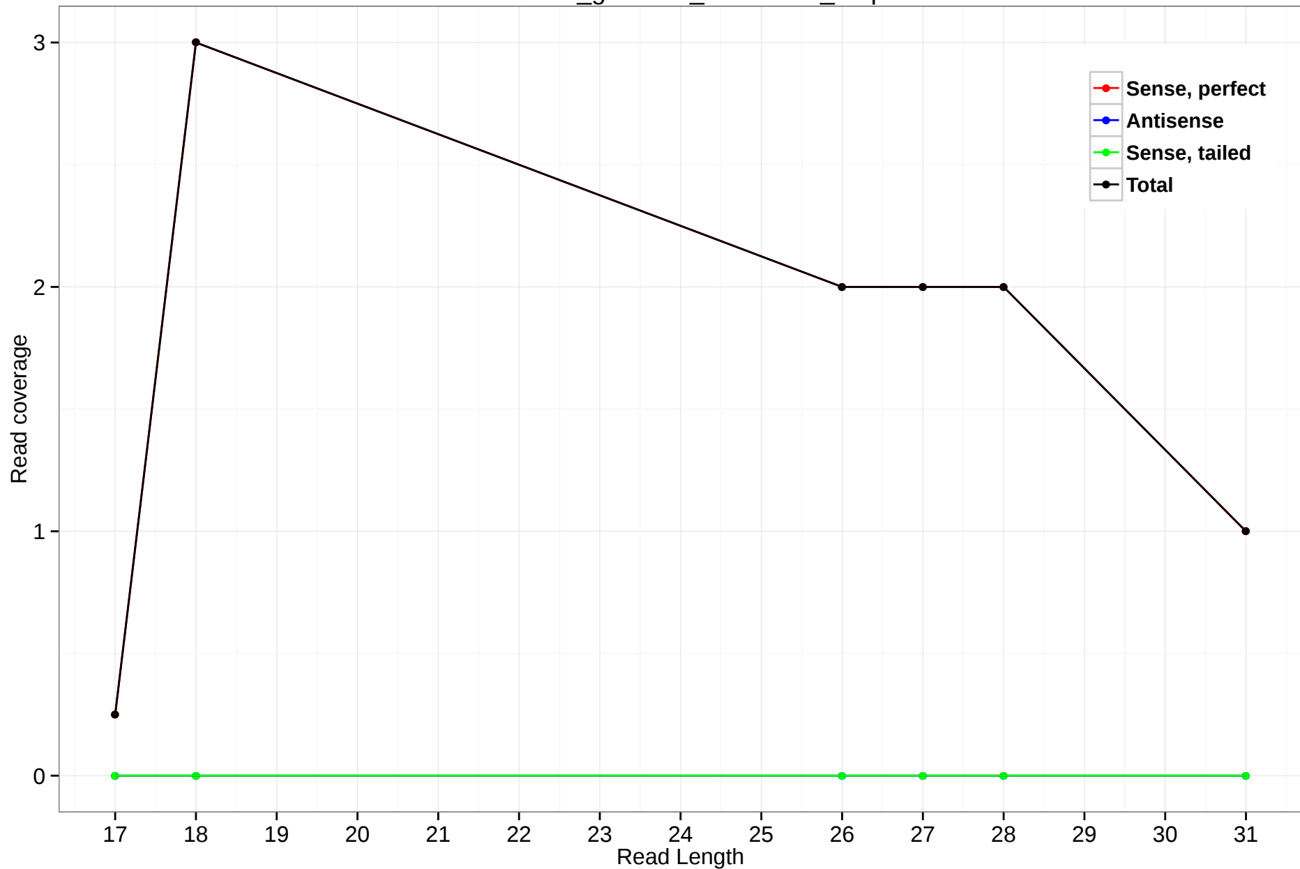
rheMac3_genscan_chr11.957_0.5p
