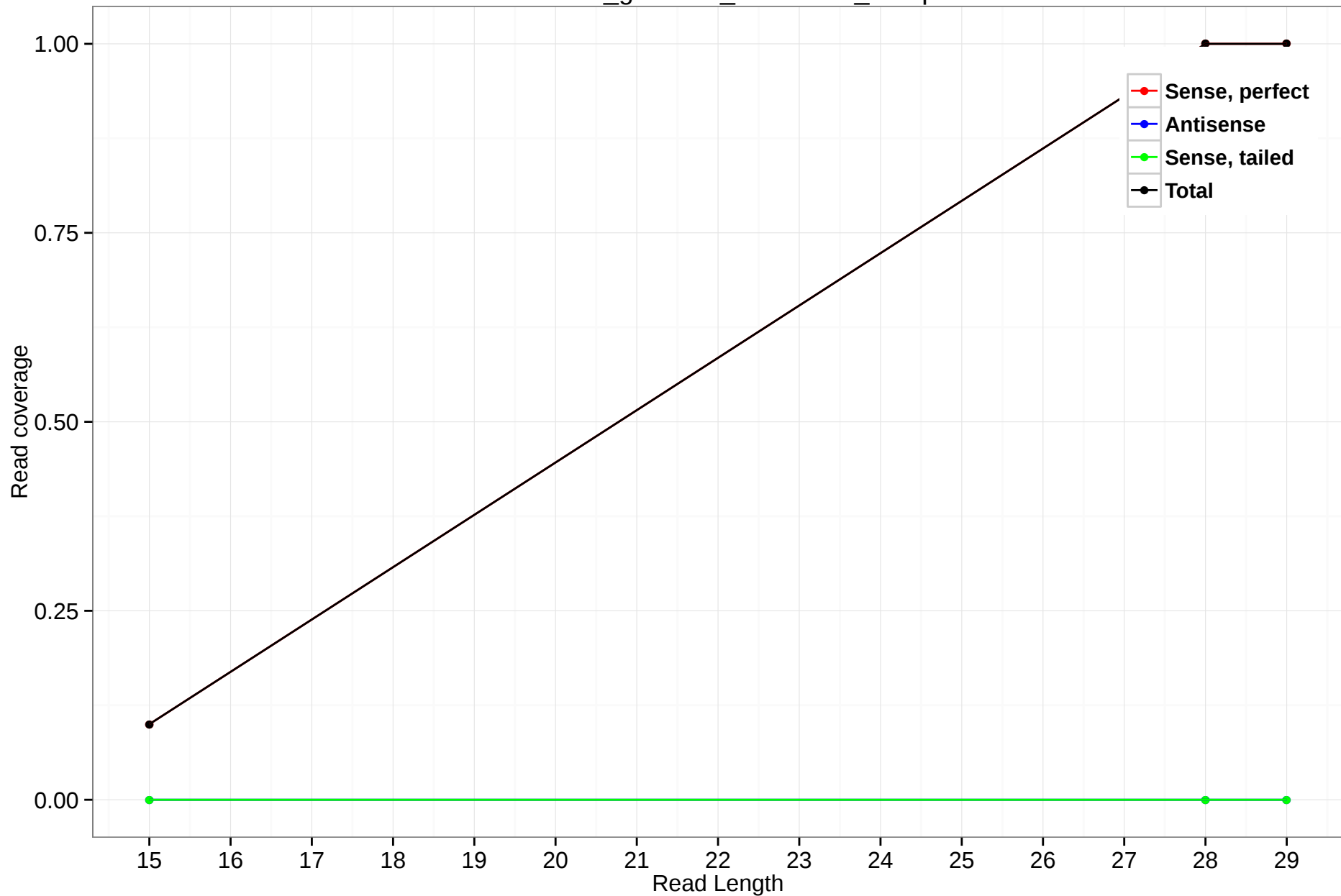
rheMac3_genscan_chr11.898_20.3p
