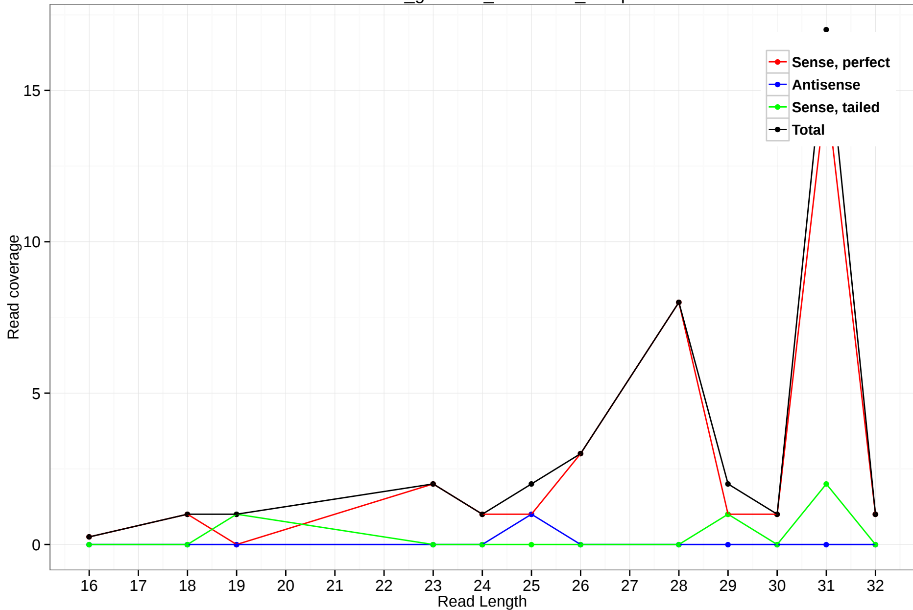
rheMac3_genscan_chr11.882_10.3p
