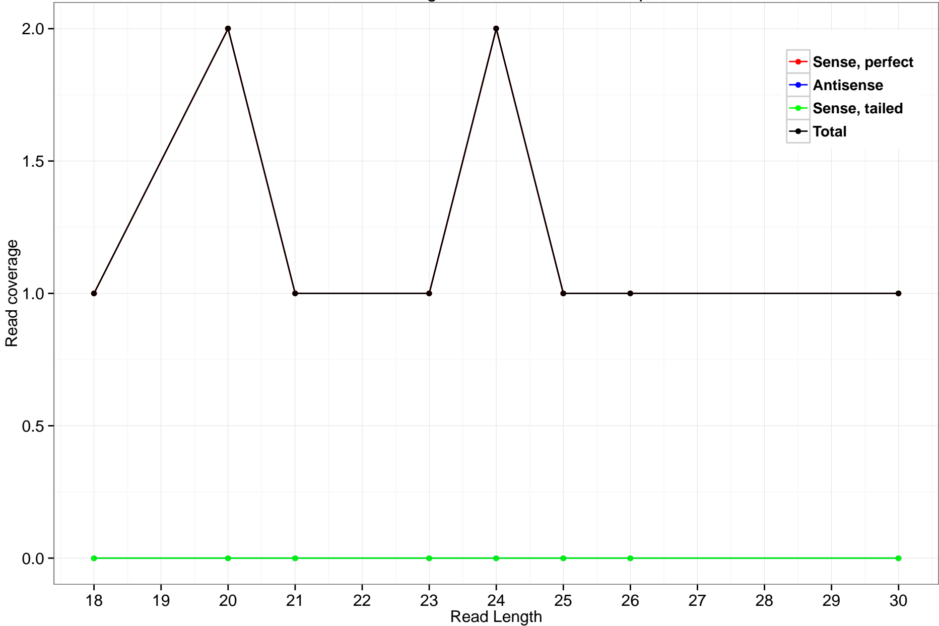
rheMac3_genscan_chr11.872_29.5p
