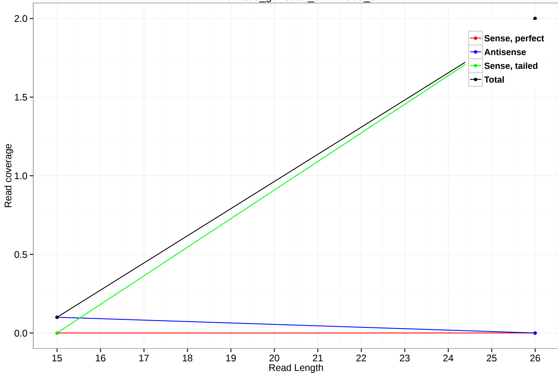
rheMac3_genscan_chr11.863_9
