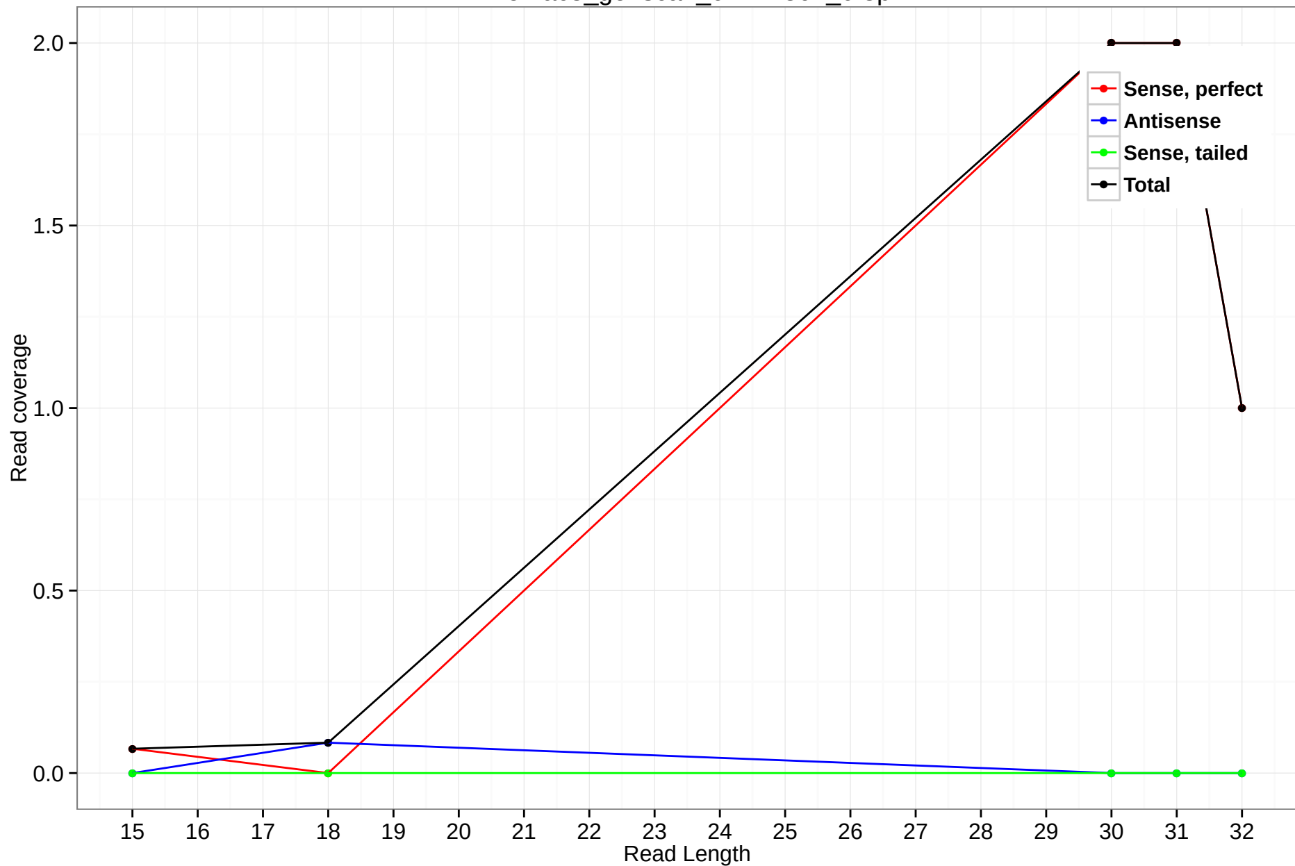
rheMac3_genscan_chr11.862_0.3p
