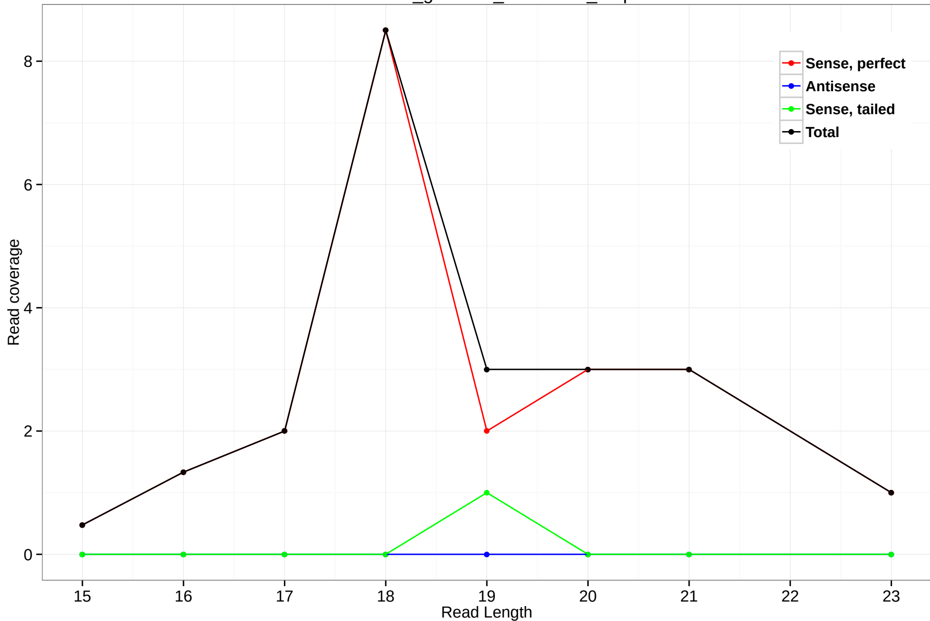
rheMac3_genscan_chr11.836_7.3p
