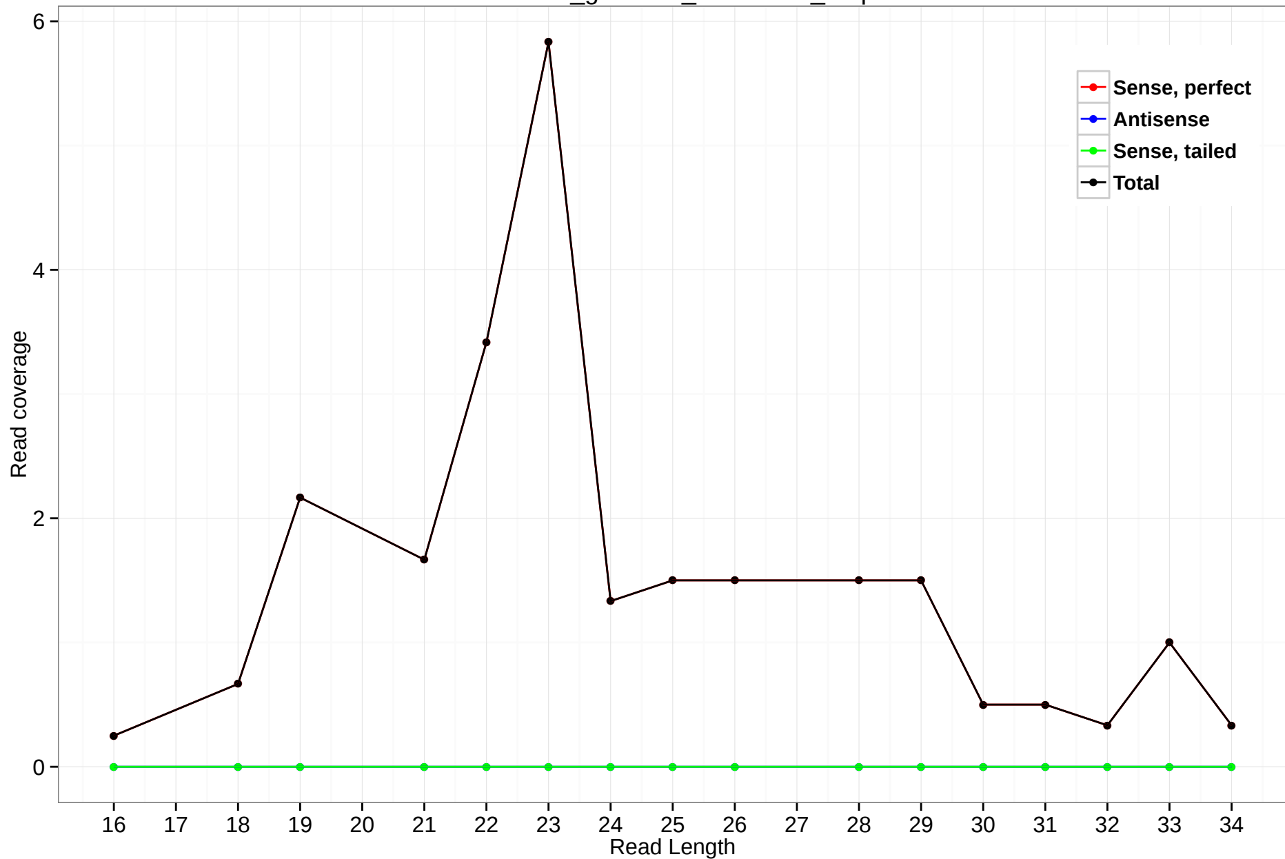
rheMac3_genscan_chr11.836_3.5p
