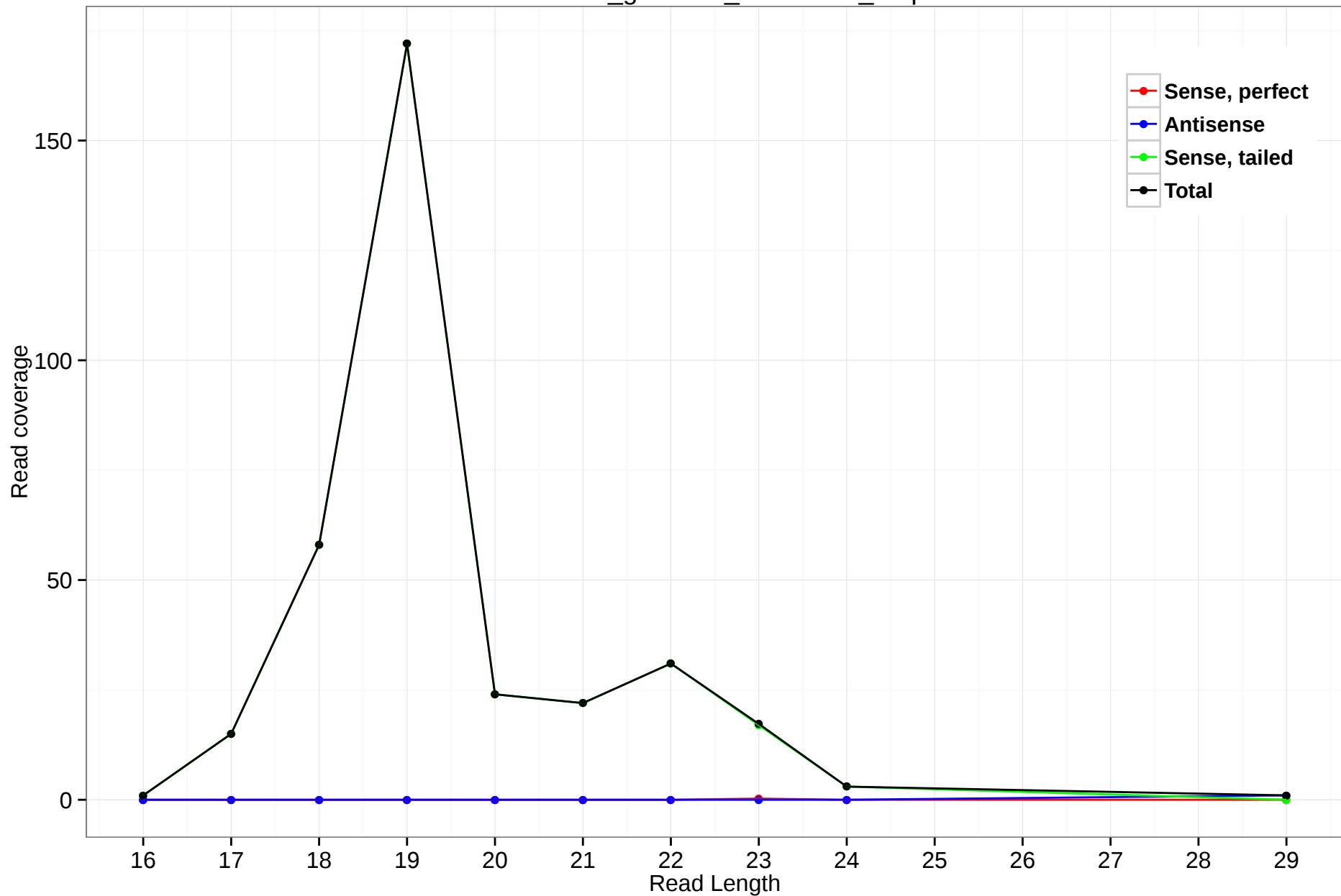
rheMac3_genscan_chr11.836_3.3p
