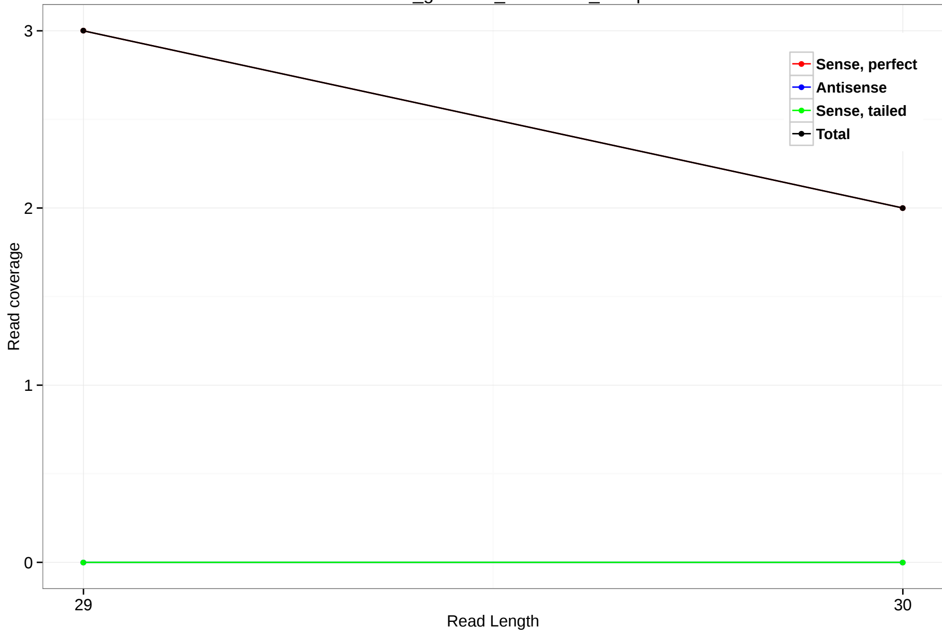
rheMac3_genscan_chr11.835_44.5p
